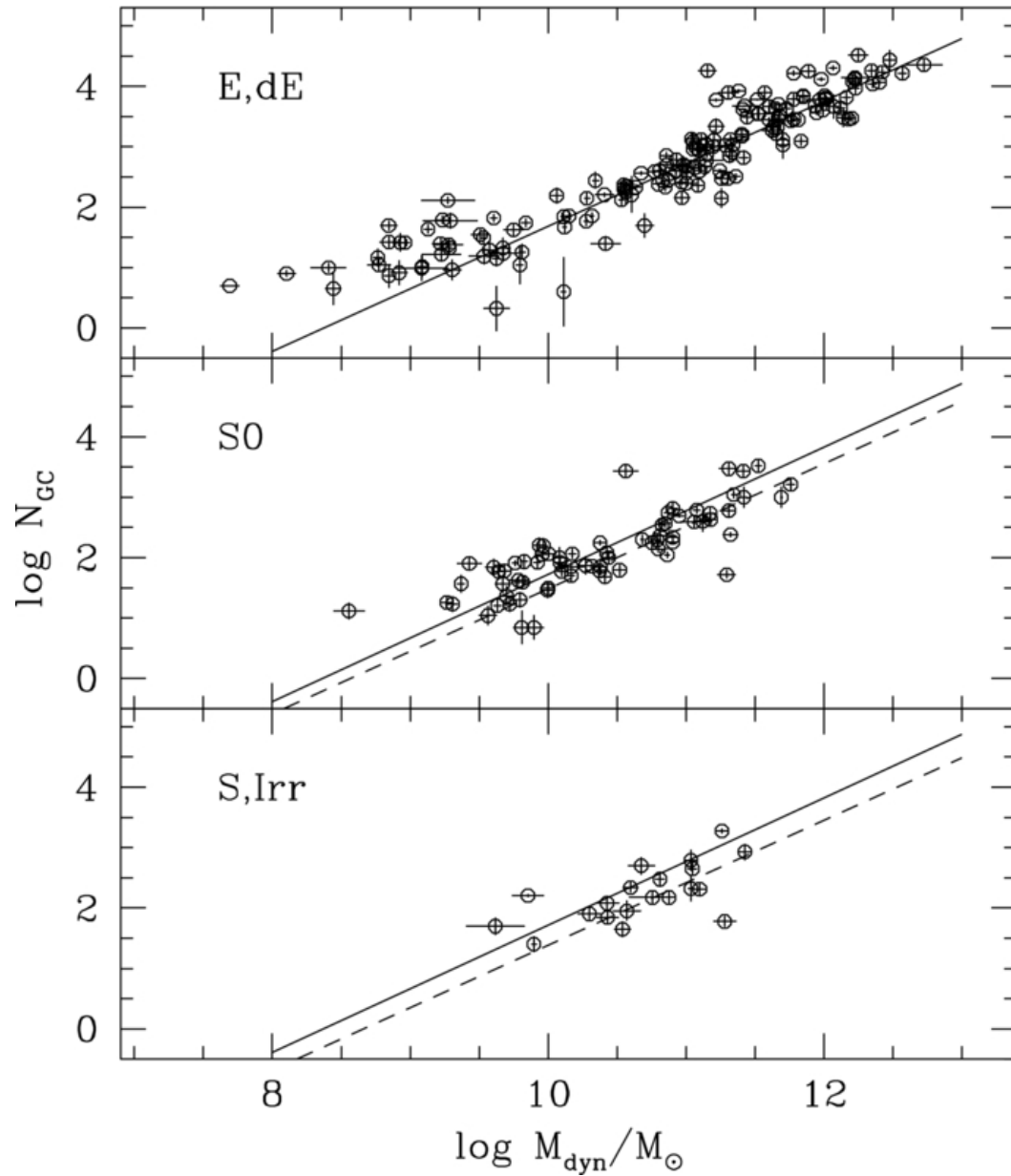
Figure 8. from A Catalog of Globular Cluster Systems: What Determines the Size of a Galaxy's Globular Cluster Population? Harris, Harris, & Alessi 2013 ApJ 772 82 doi:10.1088/0004-637X/772/2/82 https://dx.doi.org/10.1088/0004-637X/772/2/82 © 2013. The American Astronomical Society. All rights reserved.
