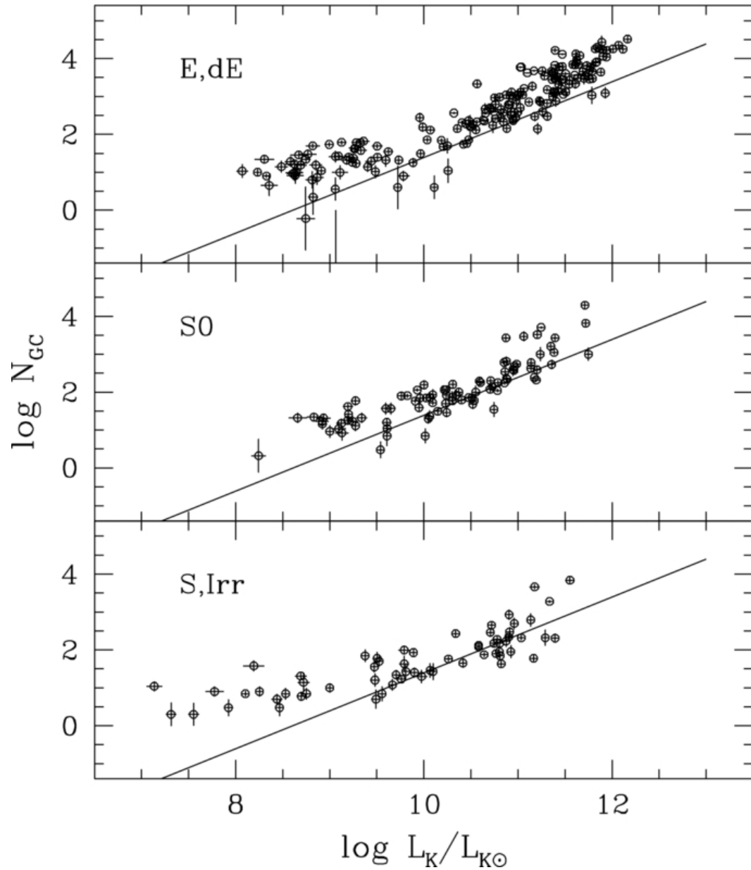
Figure 6. from A Catalog of Globular Cluster Systems: What Determines the Size of a Galaxy's Globular Cluster Population? Harris, Harris, & Alessi 2013 ApJ 772 82 doi:10.1088/0004-637X/772/2/82 https://dx.doi.org/10.1088/0004-637X/772/2/82 © 2013. The American Astronomical Society. All rights reserved.
