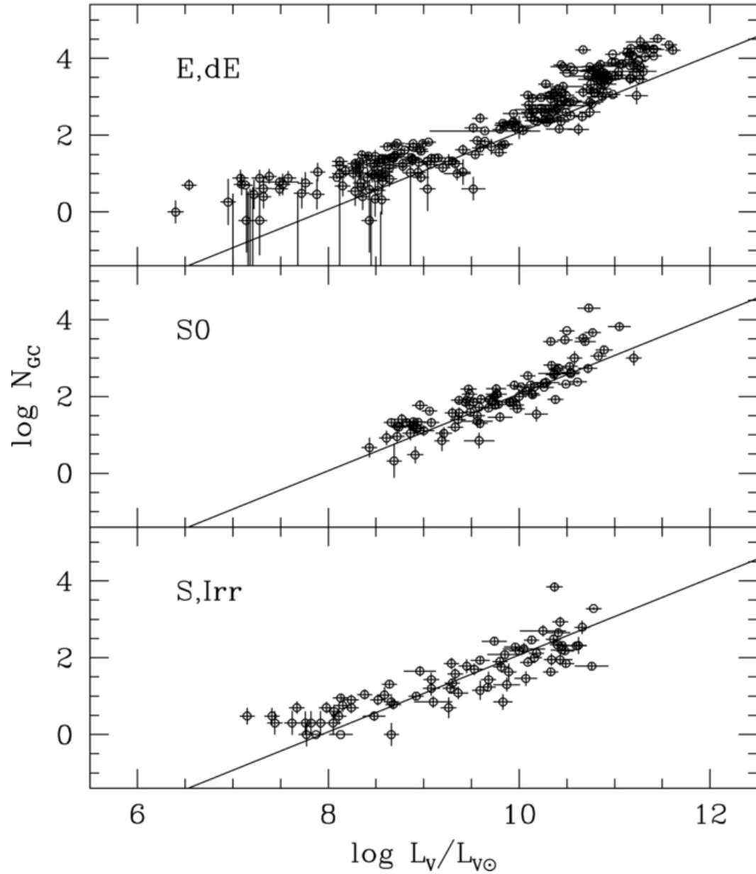
Figure 5. from A Catalog of Globular Cluster Systems: What Determines the Size of a Galaxy's Globular Cluster Population? Harris, Harris, & Alessi 2013 ApJ 772 82 doi:10.1088/0004-637X/772/2/82 https://dx.doi.org/10.1088/0004-637X/772/2/82 © 2013. The American Astronomical Society. All rights reserved.
