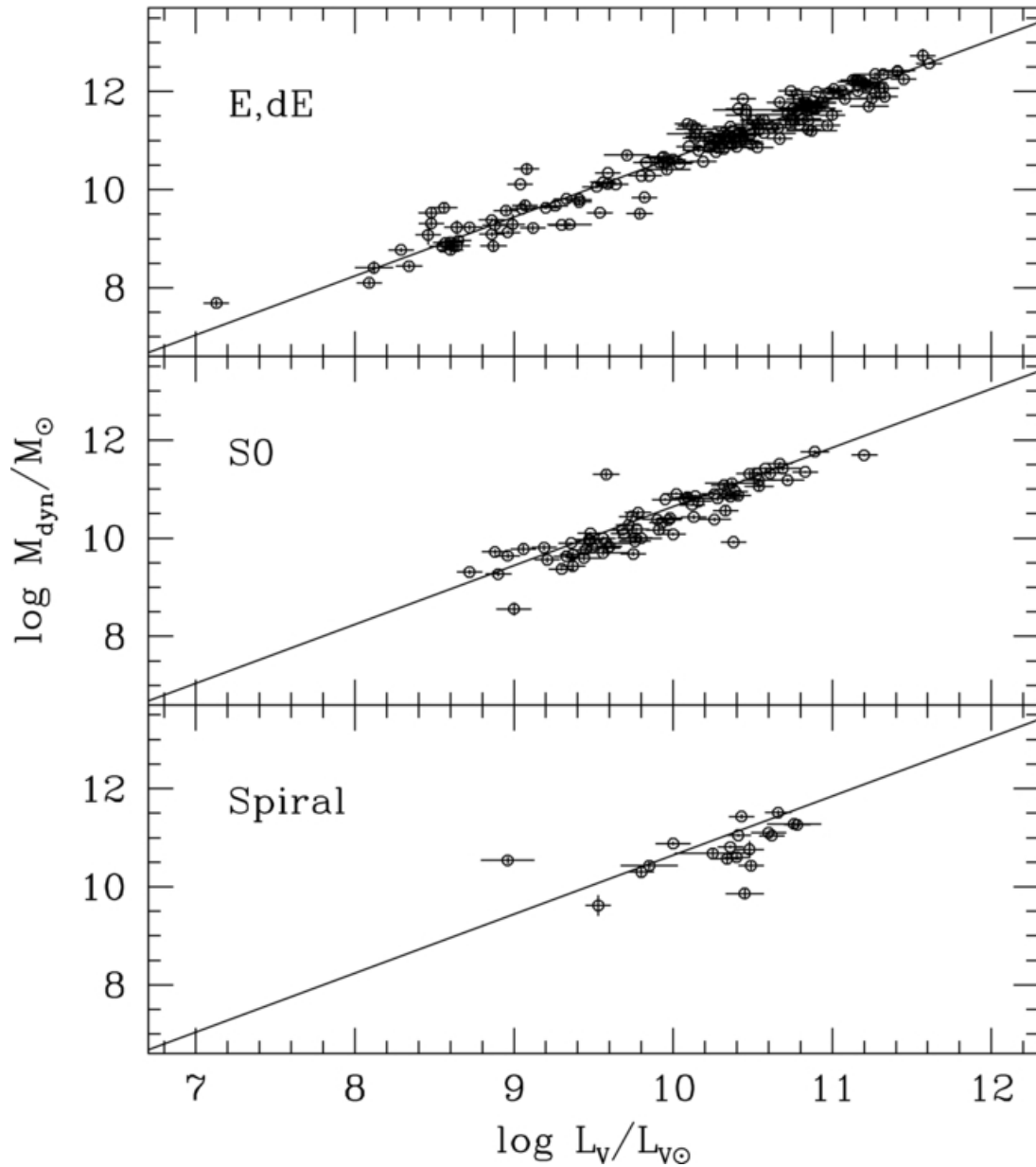
Figure 2. from A Catalog of Globular Cluster Systems: What Determines the Size of a Galaxy's Globular Cluster Population? Harris, Harris, & Alessi 2013 ApJ 772 82 doi:10.1088/0004-637X/772/2/82 https://dx.doi.org/10.1088/0004-637X/772/2/82 © 2013. The American Astronomical Society. All rights reserved.
