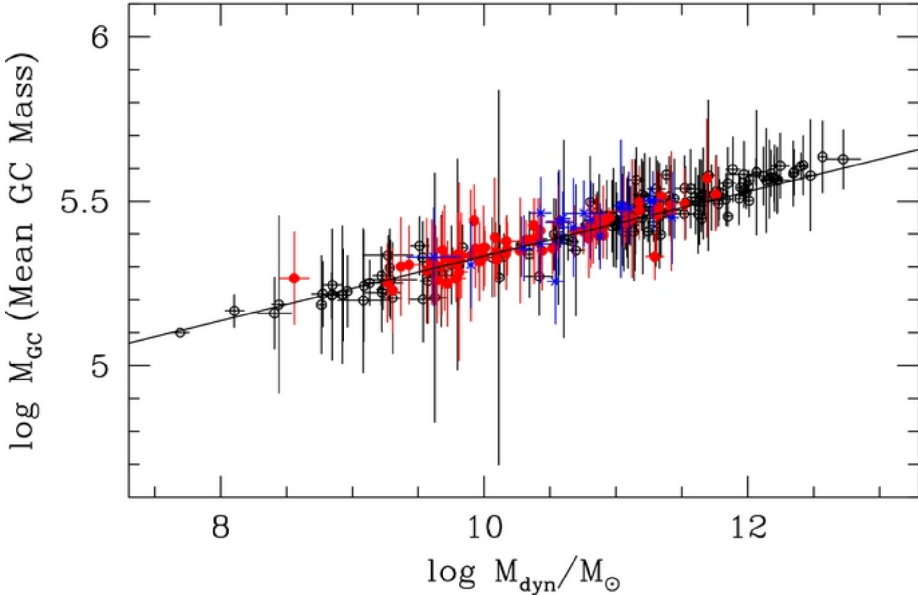
Figure 13. from A Catalog of Globular Cluster Systems: What Determines the Size of a Galaxy's Globular Cluster Population? Harris, Harris, & Alessi 2013 ApJ 772 82 doi:10.1088/0004-637X/772/2/82 https://dx.doi.org/10.1088/0004-637X/772/2/82 © 2013. The American Astronomical Society. All rights reserved.
