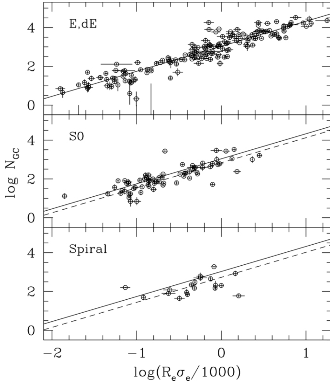
Figure 12. from A Catalog of Globular Cluster Systems: What Determines the Size of a Galaxy's Globular Cluster Population? Harris, Harris, & Alessi 2013 ApJ 772 82 doi:10.1088/0004-637X/772/2/82 https://dx.doi.org/10.1088/0004-637X/772/2/82 © 2013. The American Astronomical Society. All rights reserved.
