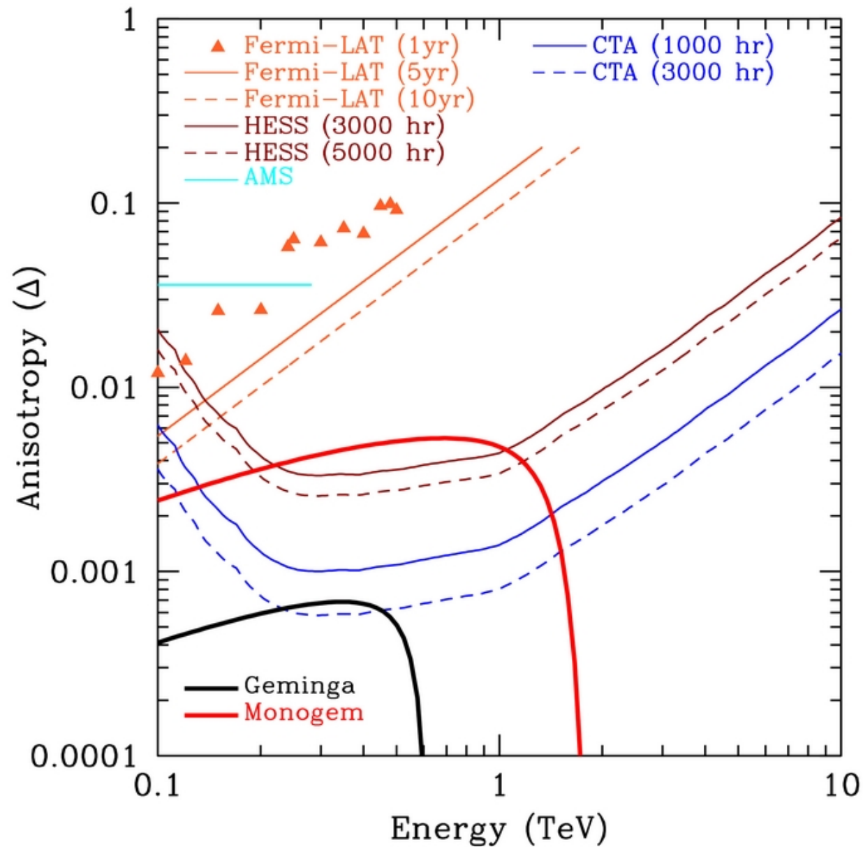
Figure 2. from Probing the Pulsar Origin of the Anomalous Positron Fraction with AMS-02 and Atmospheric Cherenkov Telescopes Linden & Profumo 2013 ApJ 772 18 doi:10.1088/0004-637X/772/1/18 https://dx.doi.org/10.1088/0004-637X/772/1/18 © 2013. The American Astronomical Society. All rights reserved.
