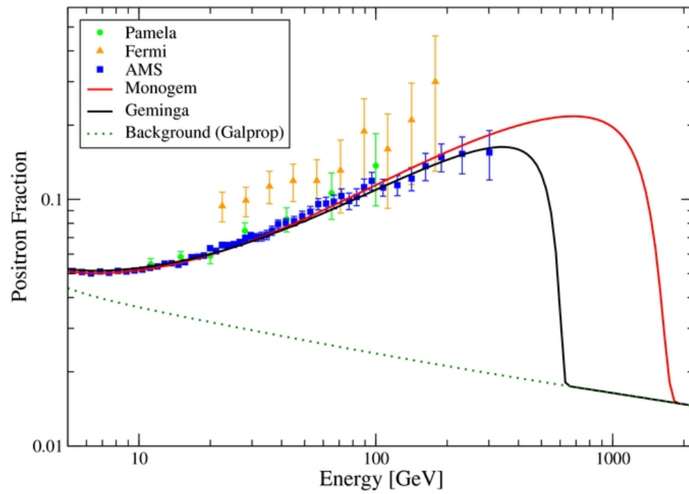
Figure 1. from Probing the Pulsar Origin of the Anomalous Positron Fraction with AMS-02 and Atmospheric Cherenkov Telescopes Linden & Profumo 2013 ApJ 772 18 doi:10.1088/0004-637X/772/1/18 https://dx.doi.org/10.1088/0004-637X/772/1/18 © 2013. The American Astronomical Society. All rights reserved.
