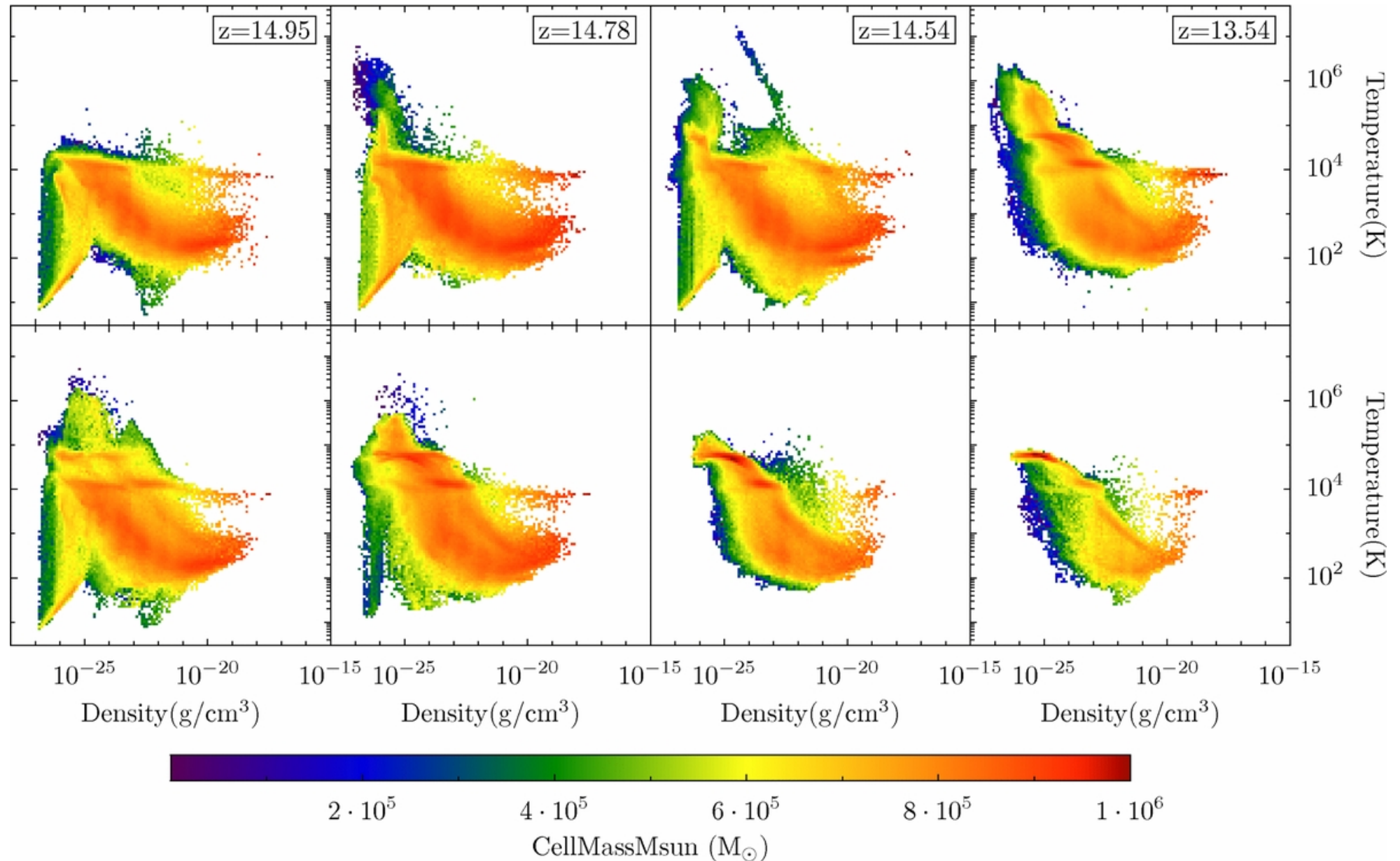
Figure 9. from The Response of Metal-rich Gas to X-Ray Irradiation from a Massive Black Hole at High Redshift: Proof of Concept Aykutalp et al. 2013 ApJ 771 50 doi:10.1088/0004-637X/771/1/50 https://dx.doi.org/10.1088/0004-637X/771/1/50 © 2013. The American Astronomical Society. All rights reserved.
