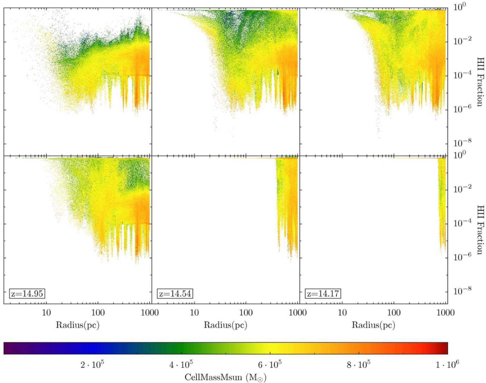
Figure 6. from The Response of Metal-rich Gas to X-Ray Irradiation from a Massive Black Hole at High Redshift: Proof of Concept Aykutaalp et al. 2013 ApJ 771 50 doi:10.1088/0004-637X/771/1/50 https://dx.doi.org/10.1088/0004-637X/771/1/50 © 2013. The American Astronomical Society. All rights reserved.
