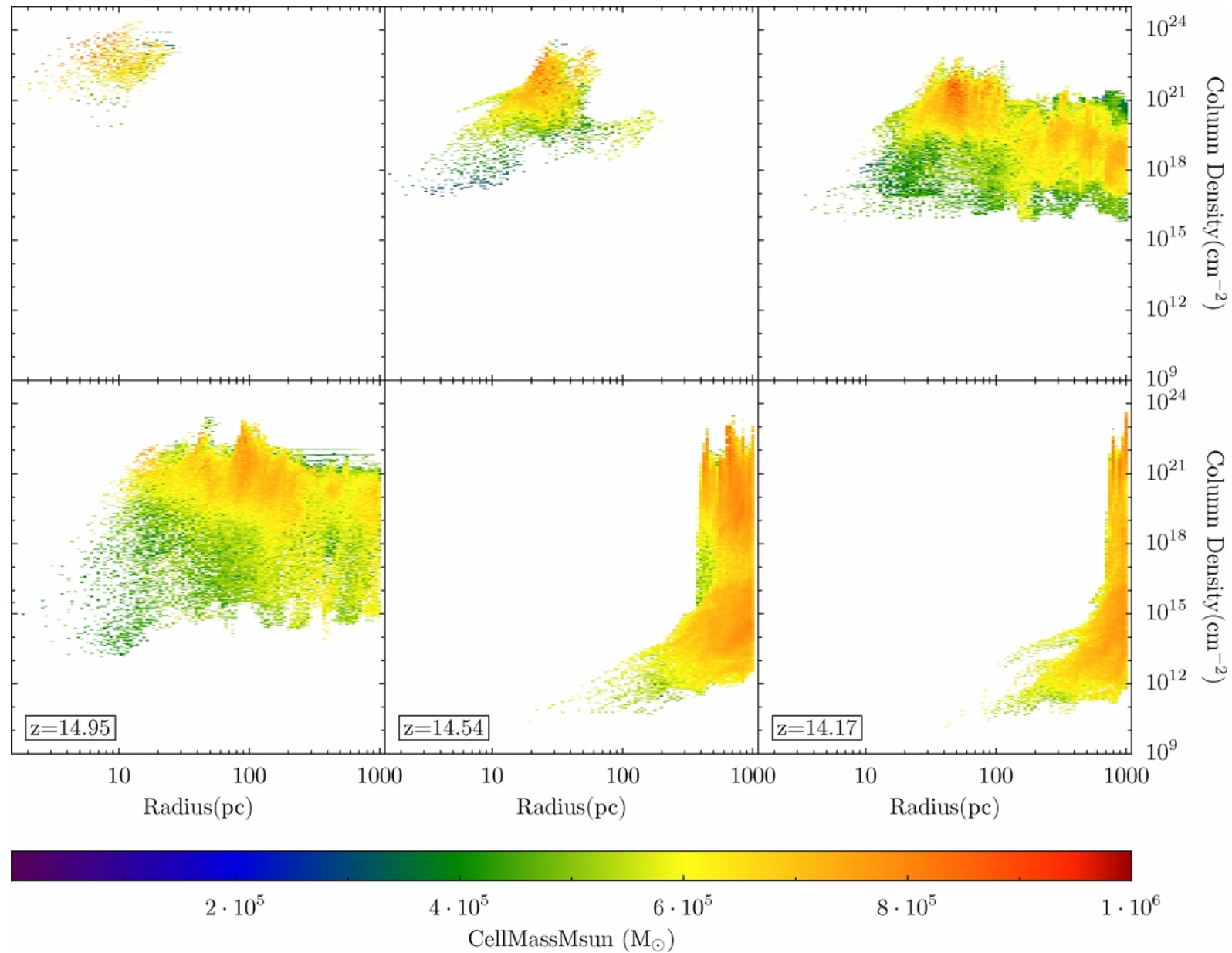
Figure 5. from The Response of Metal-rich Gas to X-Ray Irradiation from a Massive Black Hole at High Redshift: Proof of Concept Aykutaalp et al. 2013 ApJ 771 50 doi:10.1088/0004-637X/771/1/50 https://dx.doi.org/10.1088/0004-637X/771/1/50 © 2013. The American Astronomical Society. All rights reserved.
