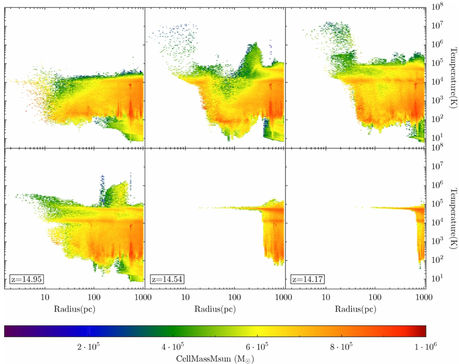
Figure 4. from The Response of Metal-rich Gas to X-Ray Irradiation from a Massive Black Hole at High Redshift: Proof of Concept Aykutaalp et al. 2013 ApJ 771 50 doi:10.1088/0004-637X/771/1/50 https://dx.doi.org/10.1088/0004-637X/771/1/50 © 2013. The American Astronomical Society. All rights reserved.
