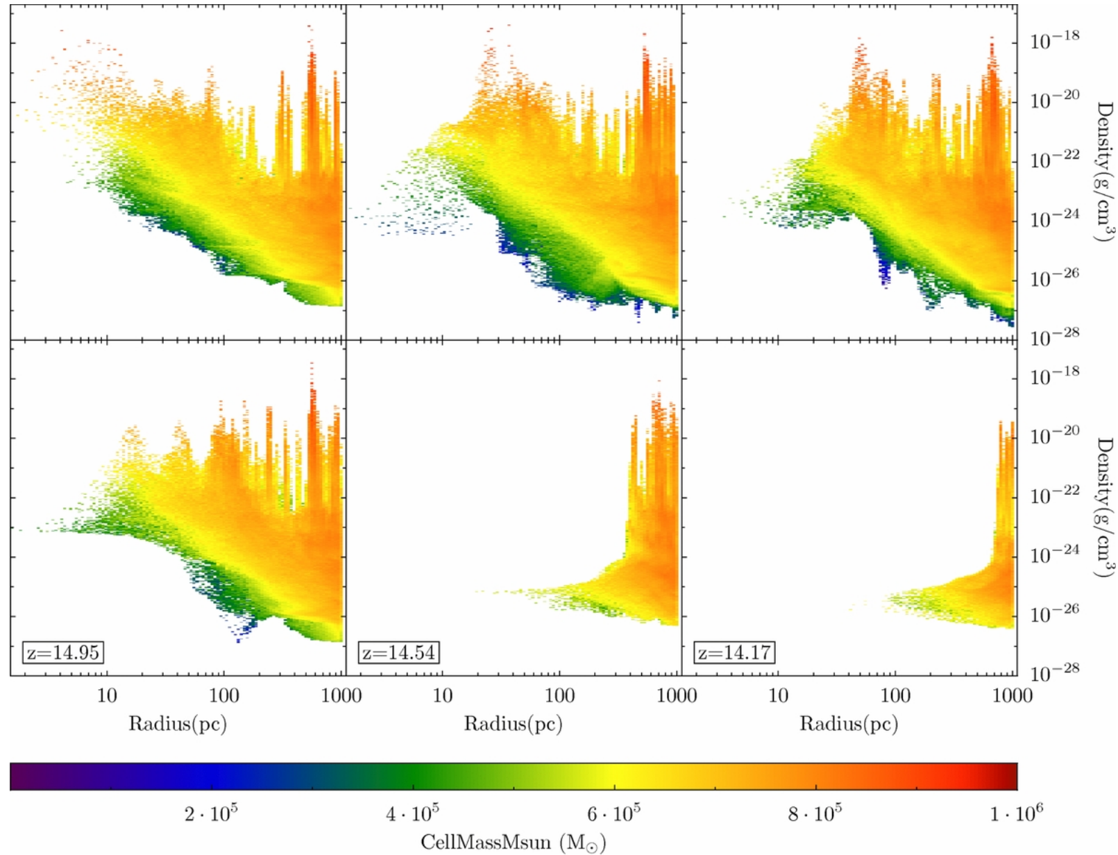
Figure 3. from The Response of Metal-rich Gas to X-Ray Irradiation from a Massive Black Hole at High Redshift: Proof of Concept Aykutaalp et al. 2013 ApJ 771 50 doi:10.1088/0004-637X/771/1/50 https://dx.doi.org/10.1088/0004-637X/771/1/50 © 2013. The American Astronomical Society. All rights reserved.
