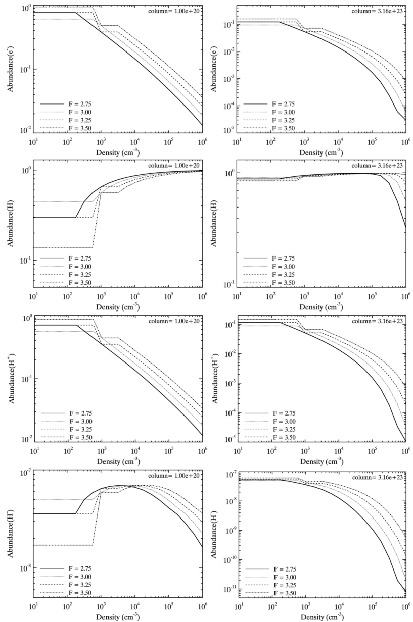
Figure 12. from The Response of Metal-rich Gas to X-Ray Irradiation from a Massive Black Hole at High Redshift: Proof of Concept Aykutalp et al. 2013 ApJ 771 50 doi:10.1088/0004-637X/771/1/50 https://dx.doi.org/10.1088/0004-637X/771/1/50
