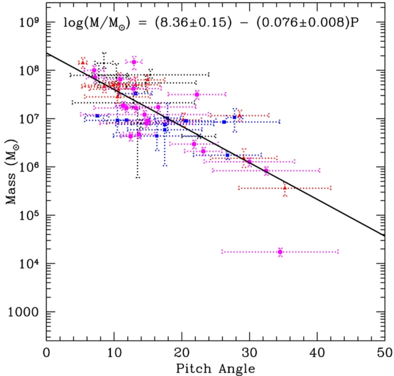
Figure 4. from Further Evidence for a Supermassive Black Hole Mass-Pitch Angle Relation Berrier et al. 2013 ApJ 769 132 doi:10.1088/0004-637X/769/2/132 https://dx.doi.org/10.1088/0004-637X/769/2/132 © 2013. The American Astronomical Society. All rights reserved.
