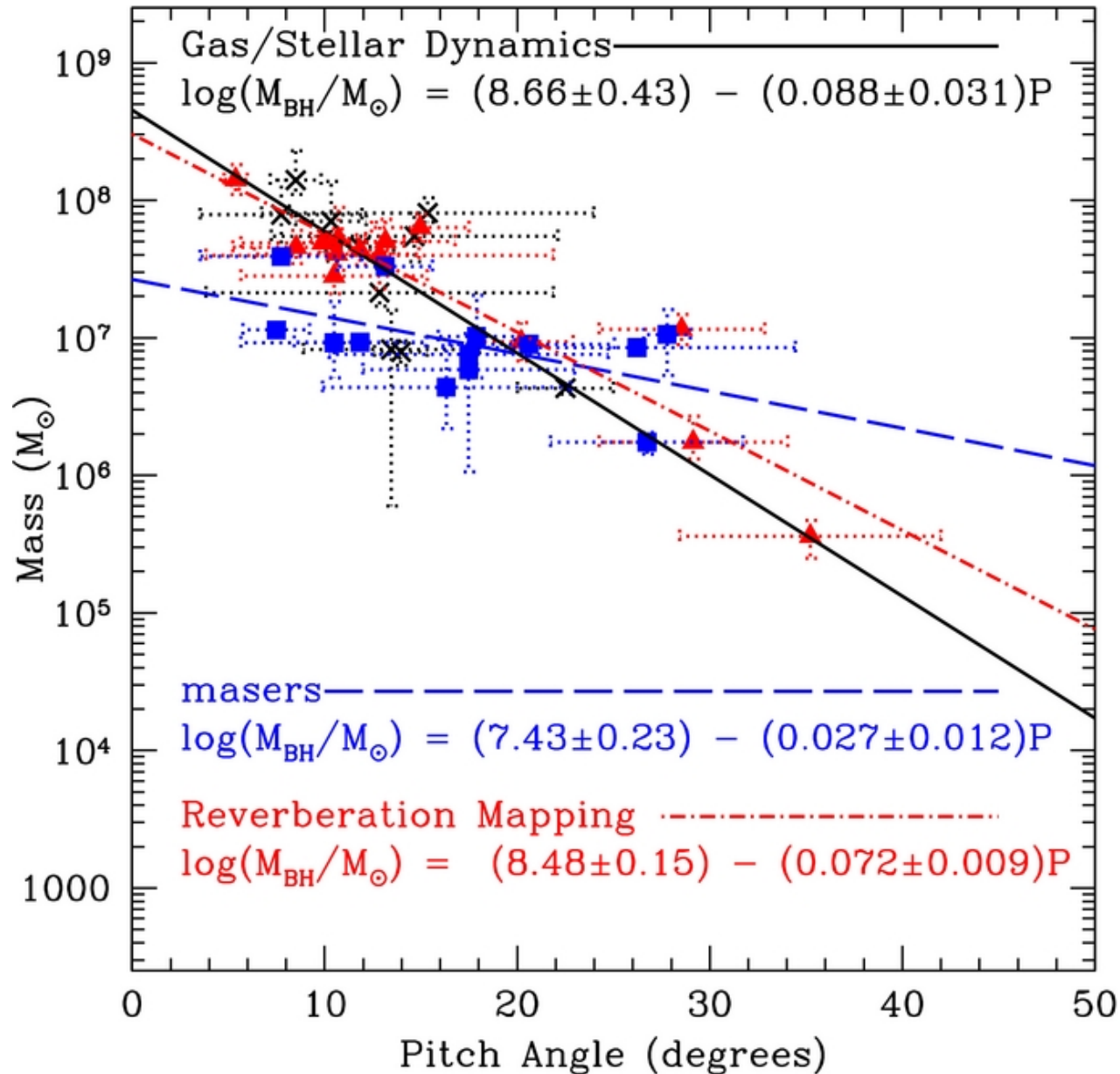
Figure 2. from Further Evidence for a Supermassive Black Hole Mass-Pitch Angle Relation Berrier et al. 2013 ApJ 769 132 doi:10.1088/0004-637X/769/2/132 https://dx.doi.org/10.1088/0004-637X/769/2/132 © 2013. The American Astronomical Society. All rights reserved.
