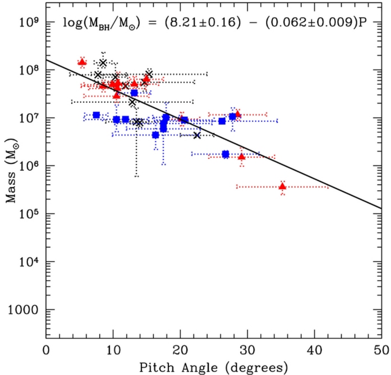
Figure 1. from Further Evidence for a Supermassive Black Hole Mass-Pitch Angle Relation Berrier et al. 2013 ApJ 769 132 doi:10.1088/0004-637X/769/2/132 https://dx.doi.org/10.1088/0004-637X/769/2/132 © 2013. The American Astronomical Society. All rights reserved.
