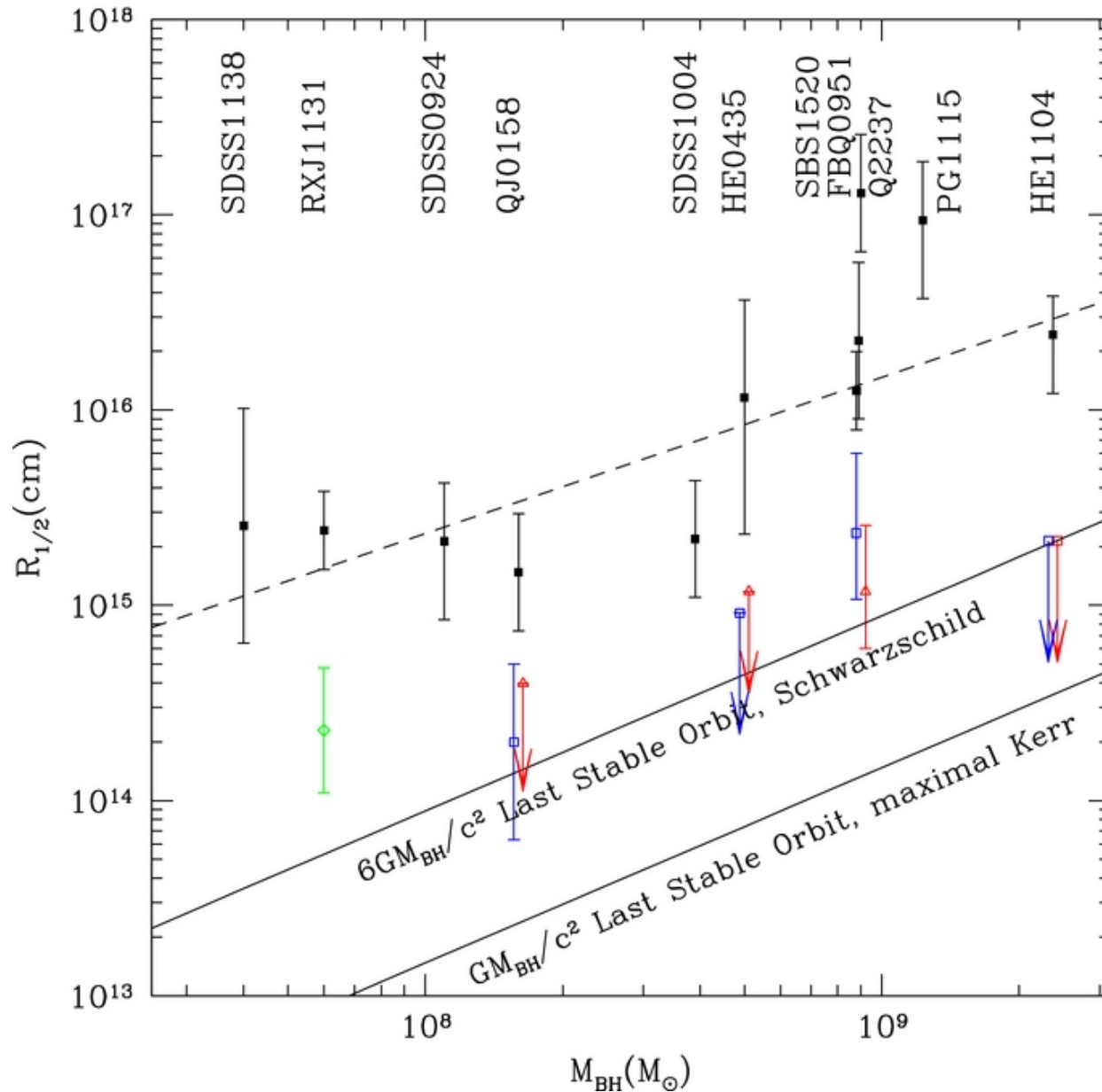
Figure 8. from The Structure of the X-Ray and Optical Emitting Regions of the Lensed Quasar Q 2237+0305 Mosquera et al. 2013 ApJ 769 53 doi:10.1088/0004-637X/769/1/53 https://dx.doi.org/10.1088/0004-637X/769/1/53 © 2013. The American Astronomical Society. All rights reserved.
