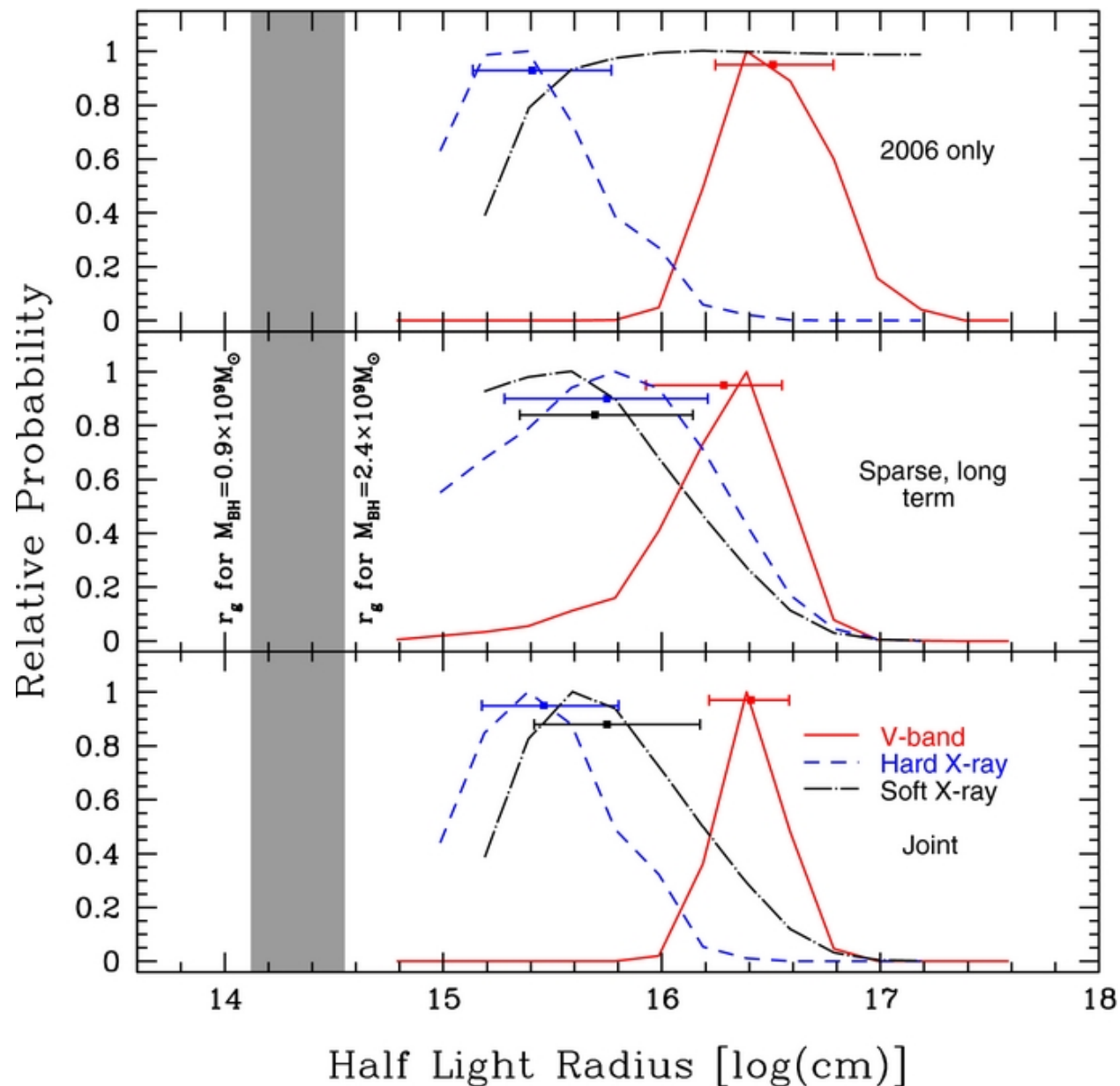
Figure 7. from The Structure of the X-Ray and Optical Emitting Regions of the Lensed Quasar Q 2237+0305 Mosquera et al. 2013 ApJ 769 53 doi:10.1088/0004-637X/769/1/53 https://dx.doi.org/10.1088/0004-637X/769/1/53 © 2013. The American Astronomical Society. All rights reserved.
