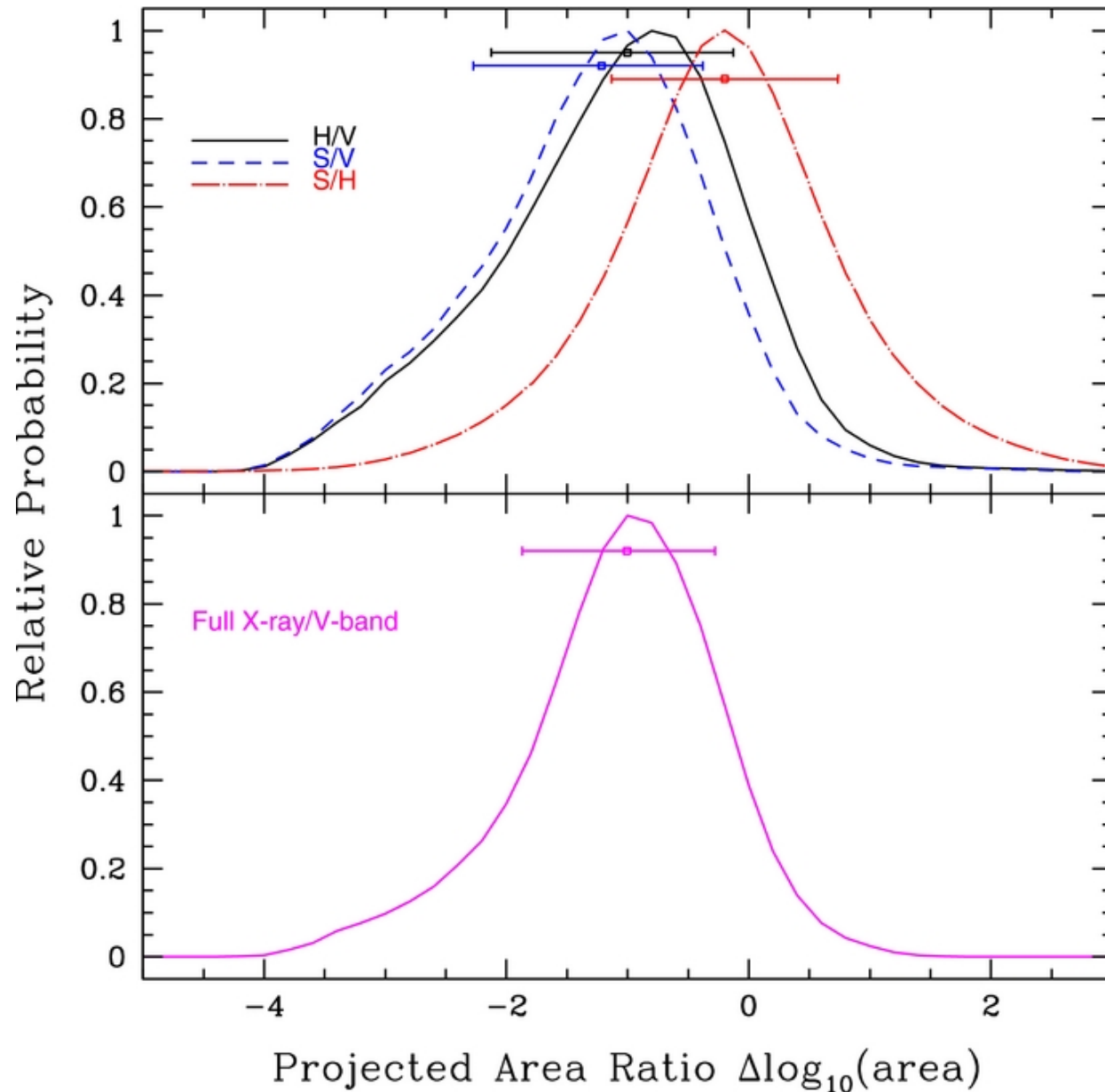
Figure 6. from The Structure of the X-Ray and Optical Emitting Regions of the Lensed Quasar Q 2237+0305 Mosquera et al. 2013 ApJ 769 53 doi:10.1088/0004-637X/769/1/53 https://dx.doi.org/10.1088/0004-637X/769/1/53 © 2013. The American Astronomical Society. All rights reserved.
