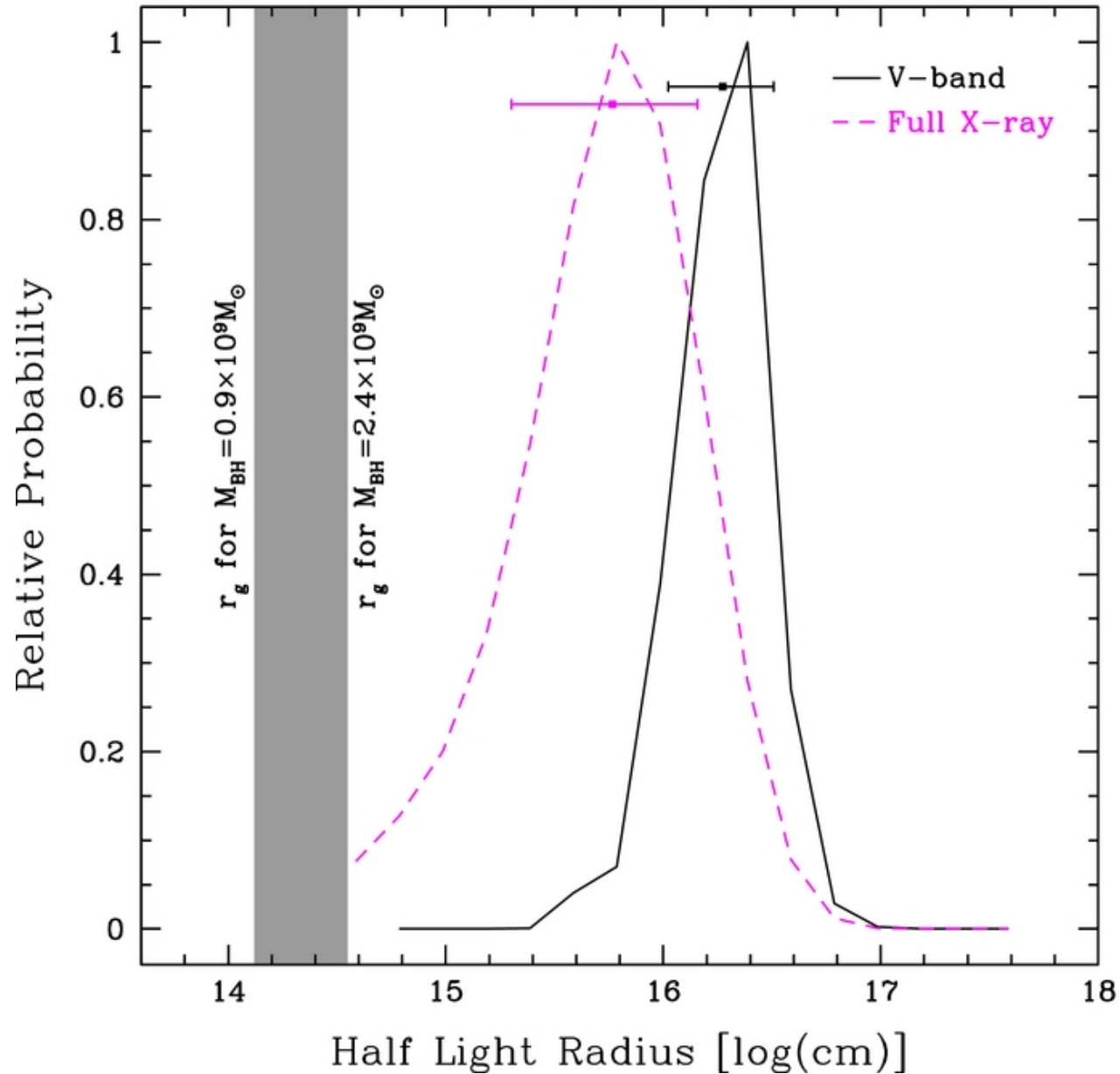
Figure 5. from The Structure of the X-Ray and Optical Emitting Regions of the Lensed Quasar Q 2237+0305 Mosquera et al. 2013 ApJ 769 53 doi:10.1088/0004-637X/769/1/53 https://dx.doi.org/10.1088/0004-637X/769/1/53 © 2013. The American Astronomical Society. All rights reserved.
