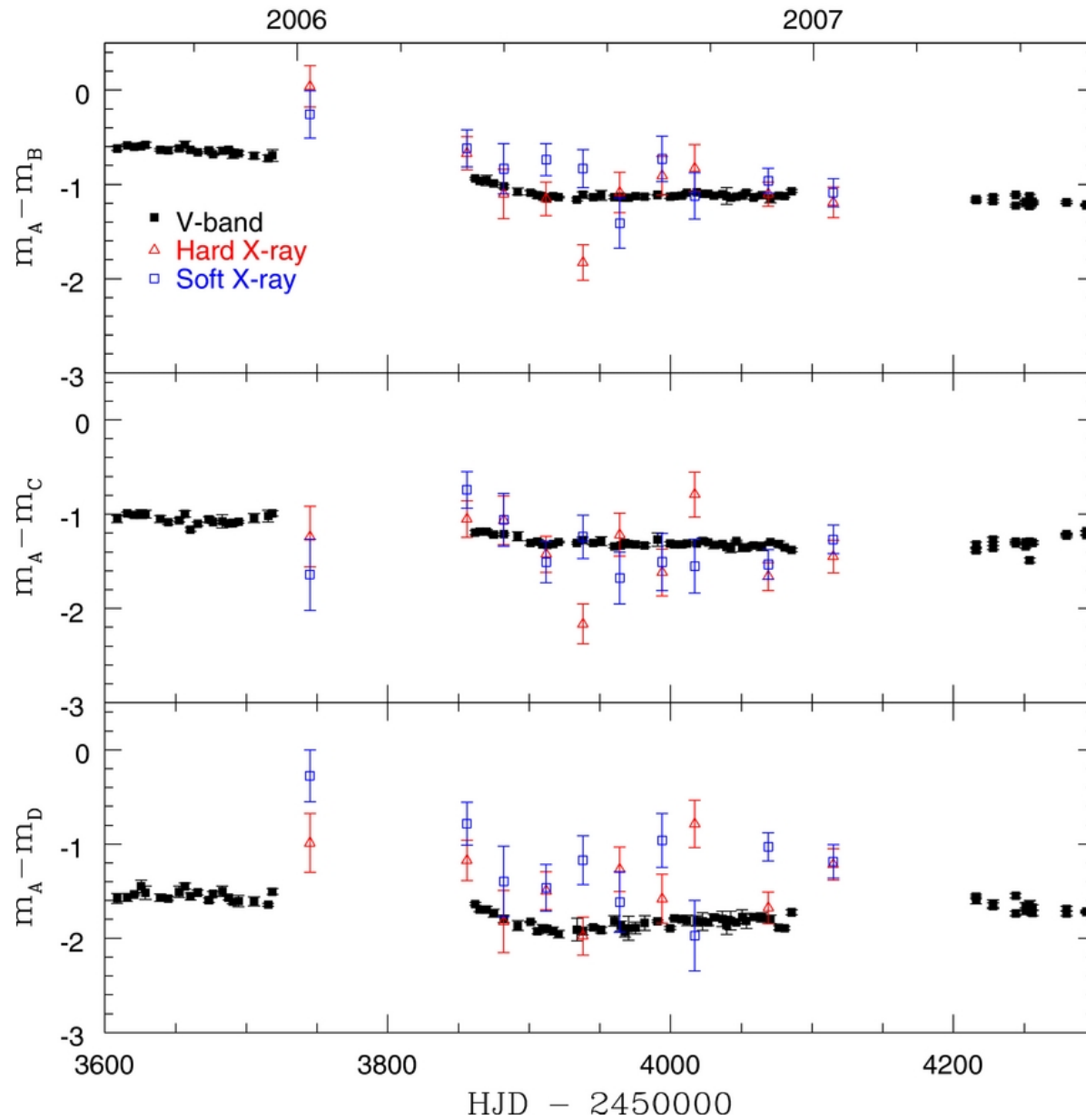
Figure 3. from The Structure of the X-Ray and Optical Emitting Regions of the Lensed Quasar Q 2237+0305 Mosquera et al. 2013 ApJ 769 53 doi:10.1088/0004-637X/769/1/53 https://dx.doi.org/10.1088/0004-637X/769/1/53 © 2013. The American Astronomical Society. All rights reserved.
