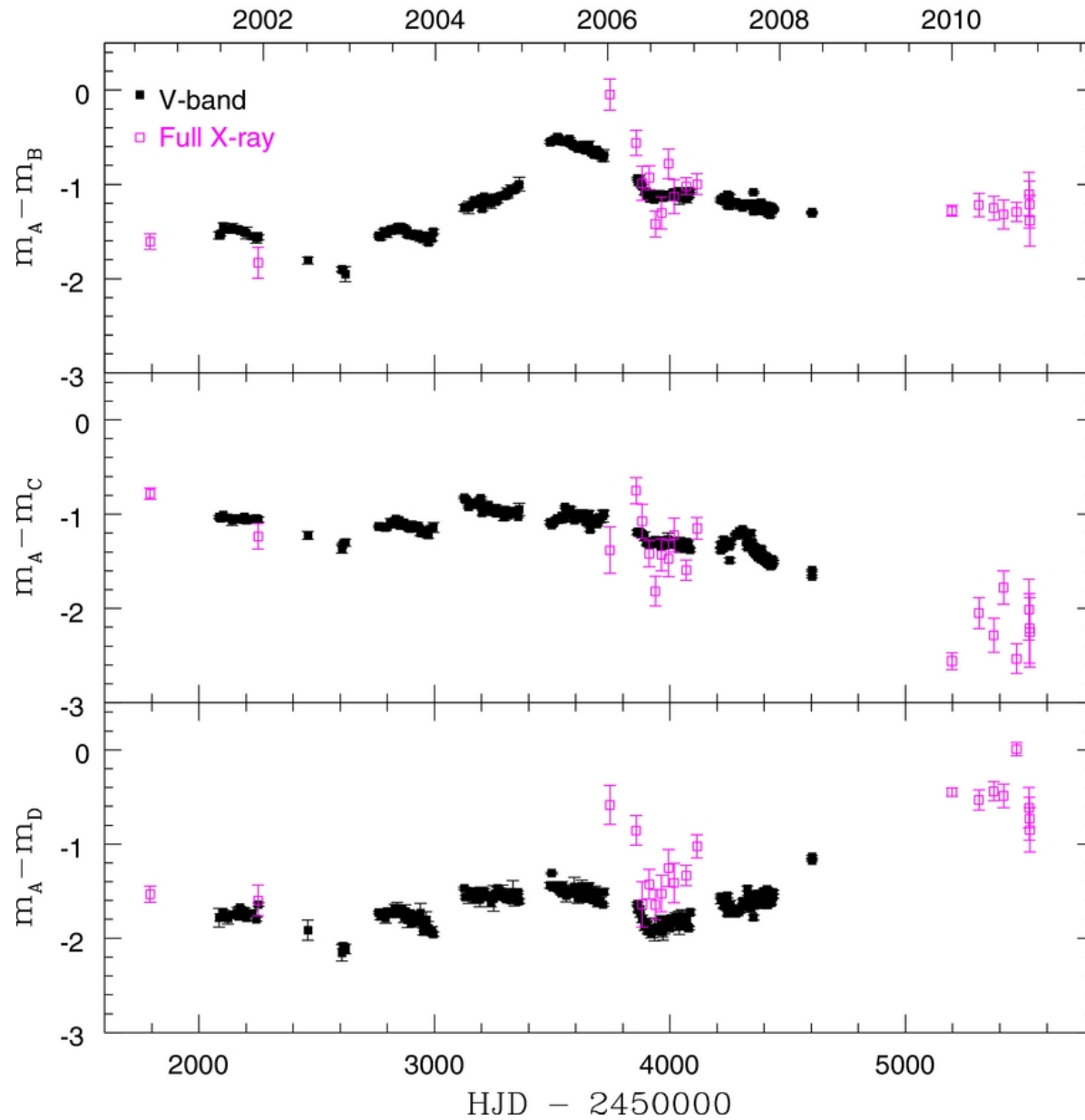
Figure 1. from The Structure of the X-Ray and Optical Emitting Regions of the Lensed Quasar Q 2237+0305 Mosquera et al. 2013 ApJ 769 53 doi:10.1088/0004-637X/769/1/53 https://dx.doi.org/10.1088/0004-637X/769/1/53 © 2013. The American Astronomical Society. All rights reserved.
