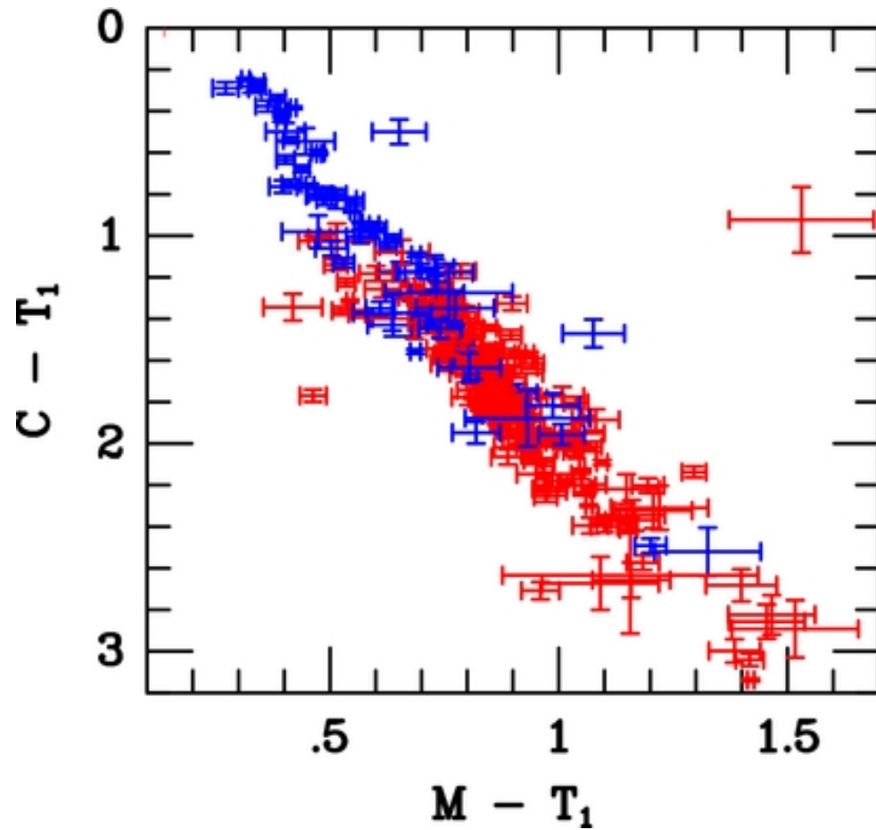
Figure 6. from A Survey for Planetary Nebulae in M31 Globular Clusters Jacoby et al. 2013 ApJ 769 10 doi:10.1088/0004-637X/769/1/10 https://dx.doi.org/10.1088/0004-637X/769/1/10 © 2013. The American Astronomical Society. All rights reserved.
