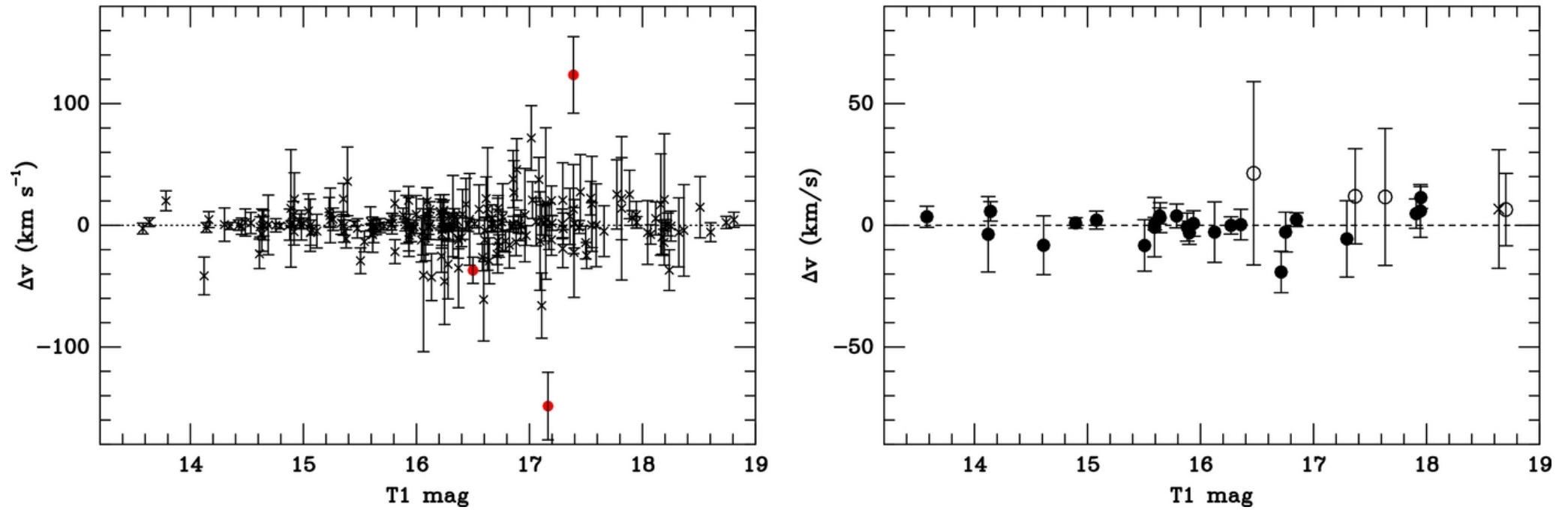
Figure 5. from A Survey for Planetary Nebulae in M31 Globular Clusters Jacoby et al. 2013 ApJ 769 10 doi:10.1088/0004-637X/769/1/10 https://dx.doi.org/10.1088/0004-637X/769/1/10 © 2013. The American Astronomical Society. All rights reserved.
