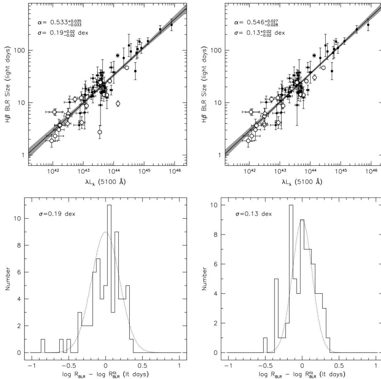
Figure 11. from The Low-luminosity End of the Radius-Luminosity Relationship for Active Galactic Nuclei Bentz et al. 2013 ApJ 767 149 doi:10.1088/0004-637X/767/2/149 https://dx.doi.org/10.1088/0004-637X/767/2/149 © 2013. The American Astronomical Society. All rights reserved.
