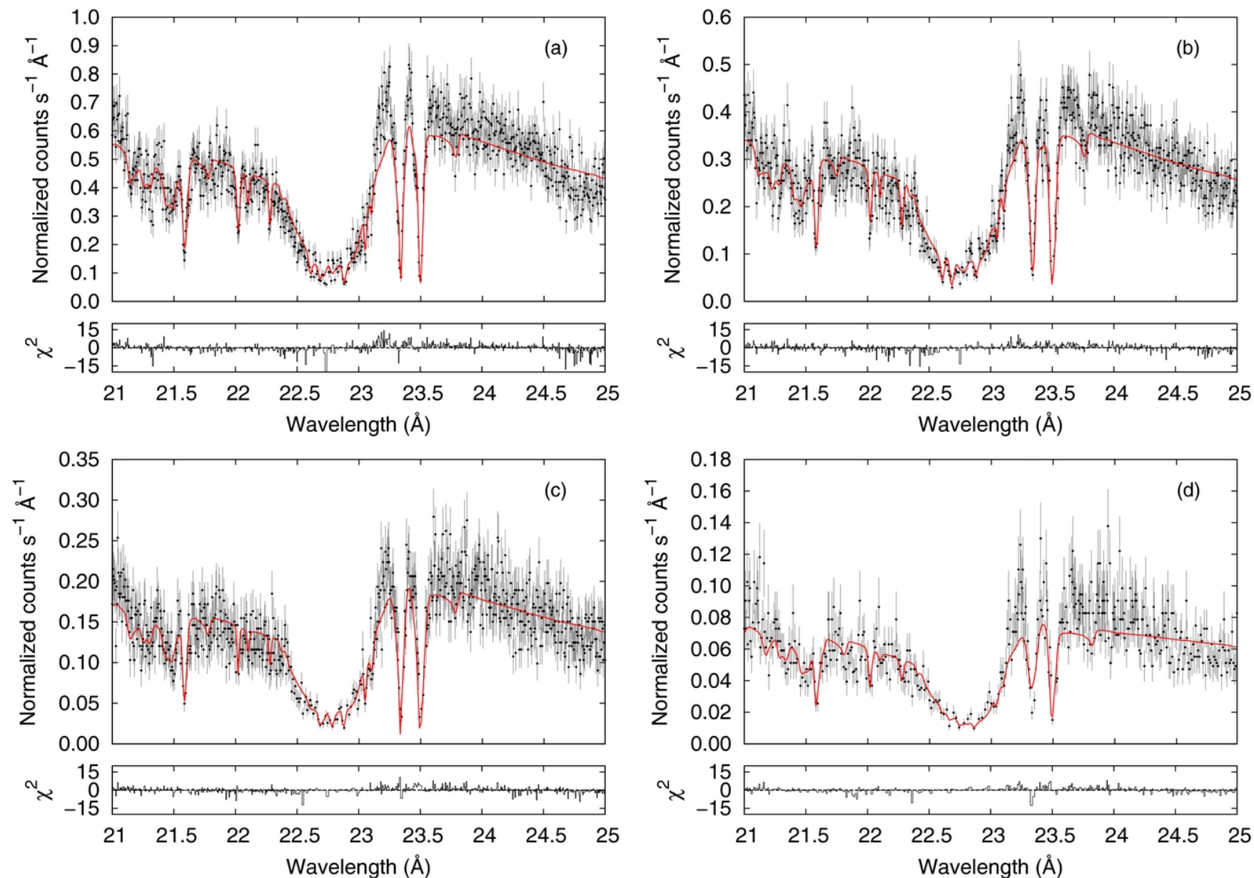
Figure 3. from Photoionization Modeling of Oxygen K Absorption in the Interstellar Medium: The Chandra Grating Spectra of XTE J1817-330 Gatuzz et al. 2013 ApJ 768 60 doi:10.1088/0004-637X/768/1/60 https://dx.doi.org/10.1088/0004-637X/768/1/60 © 2013. The American Astronomical Society. All rights reserved.
