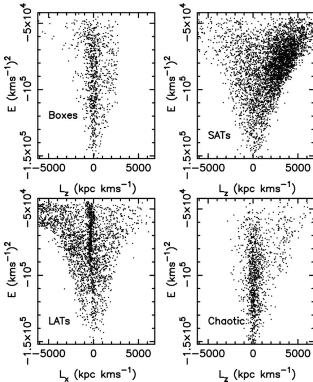
Figure 7. from Halo Orbits in Cosmological Disk Galaxies: Tracers of Formation History Valluri et al. 2013 ApJ 767 93 doi:10.1088/0004-637X/767/1/93 https://dx.doi.org/10.1088/0004-637X/767/1/93 © 2013. The American Astronomical Society. All rights reserved.
