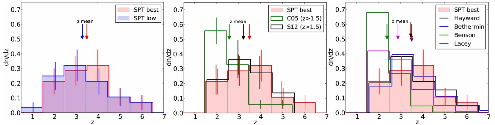
Figure 9. from ALMA Redshifts of Millimeter-selected Galaxies from the SPT Survey: The Redshift Distribution of Dusty Star-forming Galaxies Weiß et al. 2013 ApJ 767 88 doi:10.1088/0004-637X/767/1/88 https://dx.doi.org/10.1088/0004-637X/767/1/88 © 2013. The American Astronomical Society. All rights reserved.
