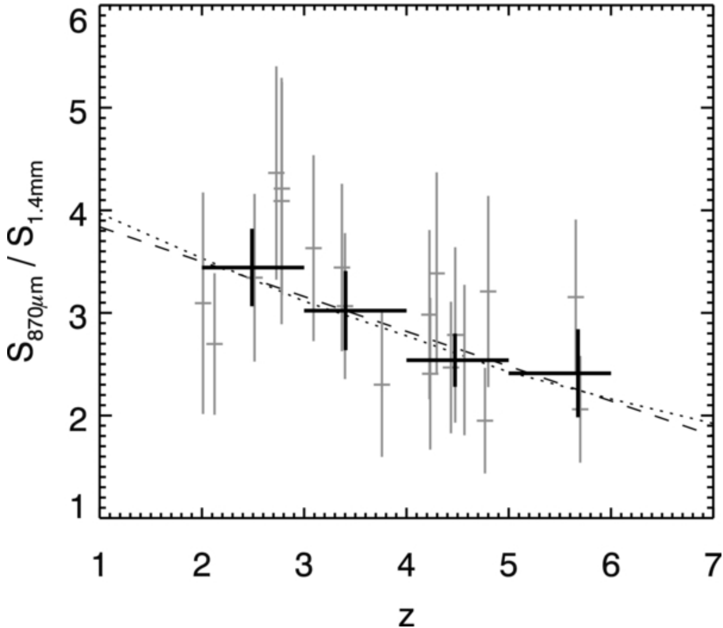
Figure 8. from ALMA Redshifts of Millimeter-selected Galaxies from the SPT Survey: The Redshift Distribution of Dusty Star-forming Galaxies Weiß et al. 2013 ApJ 767 88 doi:10.1088/0004-637X/767/1/88 https://dx.doi.org/10.1088/0004-637X/767/1/88 © 2013. The American Astronomical Society. All rights reserved.
