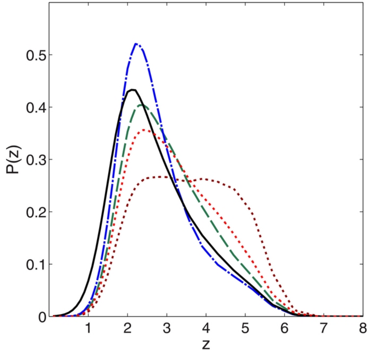
Figure 7. from ALMA Redshifts of Millimeter-selected Galaxies from the SPT Survey: The Redshift Distribution of Dusty Star-forming Galaxies Weiß et al. 2013 ApJ 767 88 doi:10.1088/0004-637X/767/1/88 https://dx.doi.org/10.1088/0004-637X/767/1/88 © 2013. The American Astronomical Society. All rights reserved.
