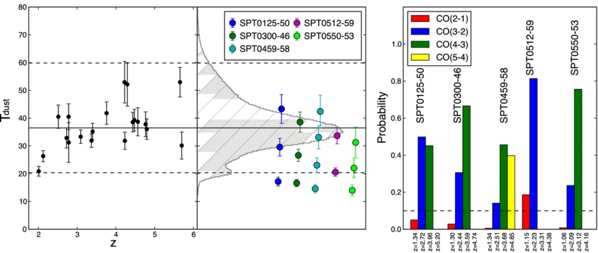
Figure 4. from ALMA Redshifts of Millimeter-selected Galaxies from the SPT Survey: The Redshift Distribution of Dusty Star-forming Galaxies Weiß et al. 2013 ApJ 767 88 doi:10.1088/0004-637X/767/1/88 https://dx.doi.org/10.1088/0004-637X/767/1/88 © 2013. The American Astronomical Society. All rights reserved.
