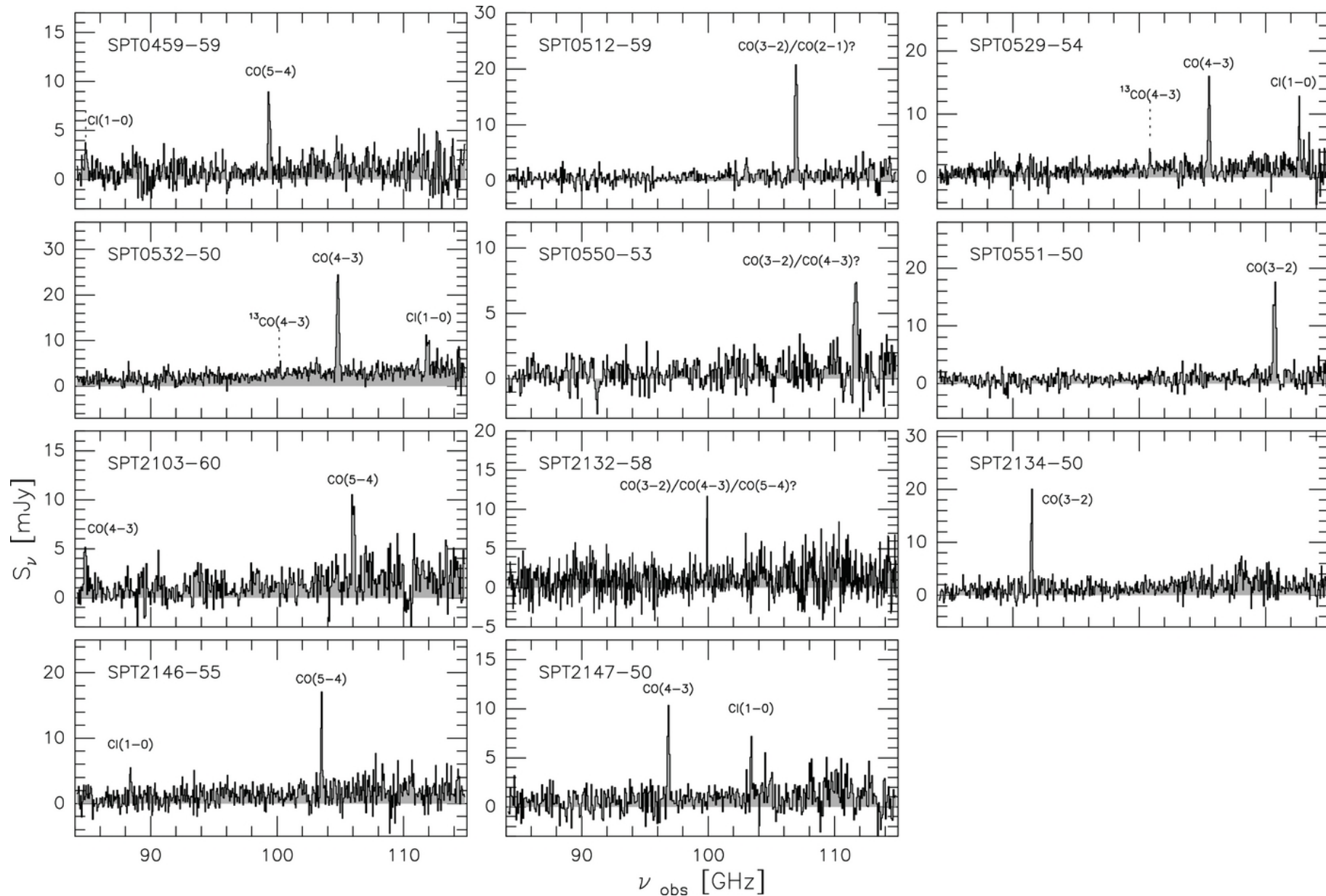
Figure 3. from ALMA Redshifts of Millimeter-selected Galaxies from the SPT Survey: The Redshift Distribution of Dusty Star-forming Galaxies Weiß et al. 2013 ApJ 767 88 doi:10.1088/0004-637X/767/1/88 https://dx.doi.org/10.1088/0004-637X/767/1/88 © 2013. The American Astronomical Society. All rights reserved.
