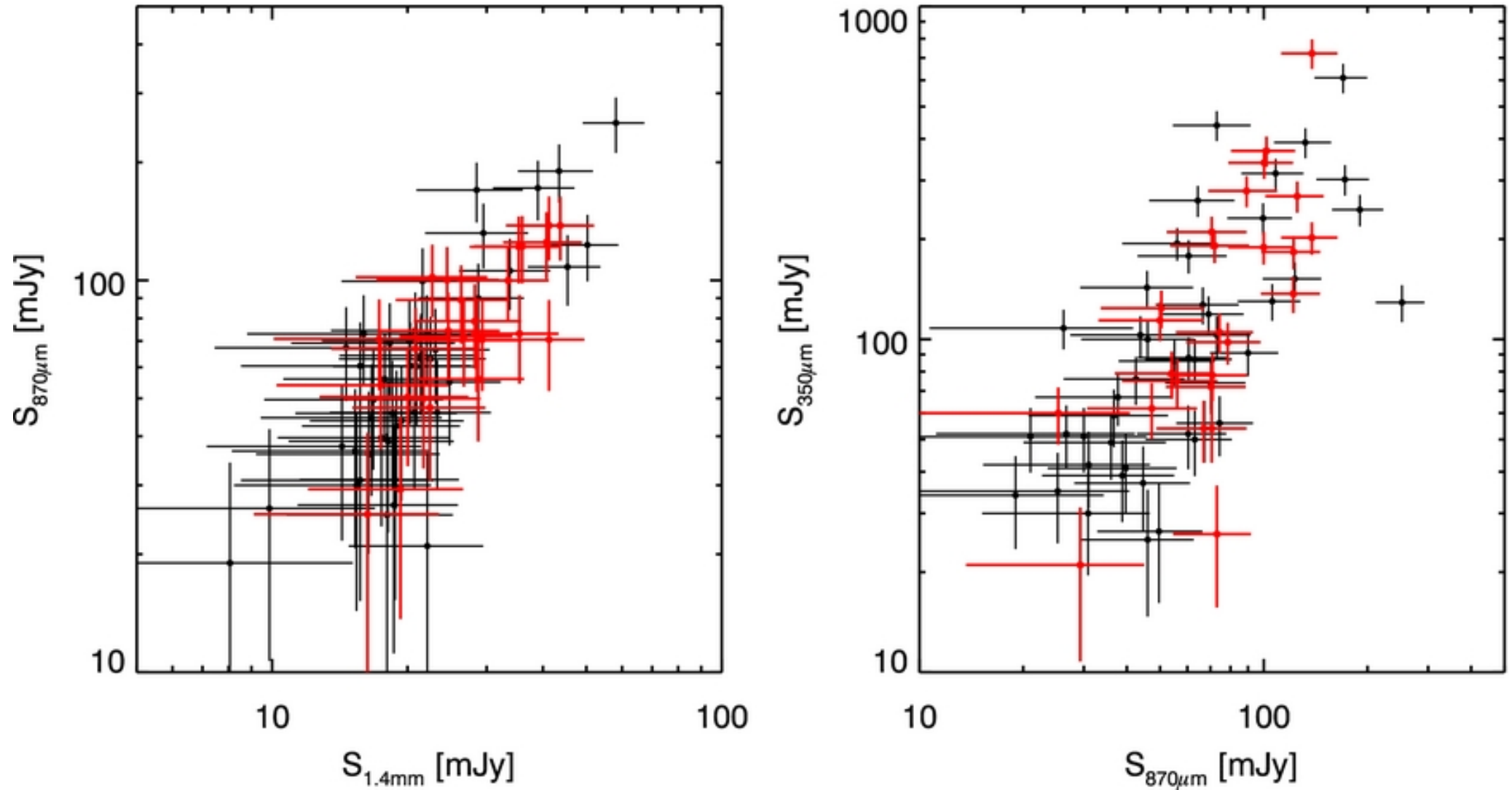
Figure 16. from ALMA Redshifts of Millimeter-selected Galaxies from the SPT Survey: The Redshift Distribution of Dusty Star-forming Galaxies Weiß et al. 2013 ApJ 767 88 doi:10.1088/0004-637X/767/1/88 https://dx.doi.org/10.1088/0004-637X/767/1/88 © 2013. The American Astronomical Society. All rights reserved.
