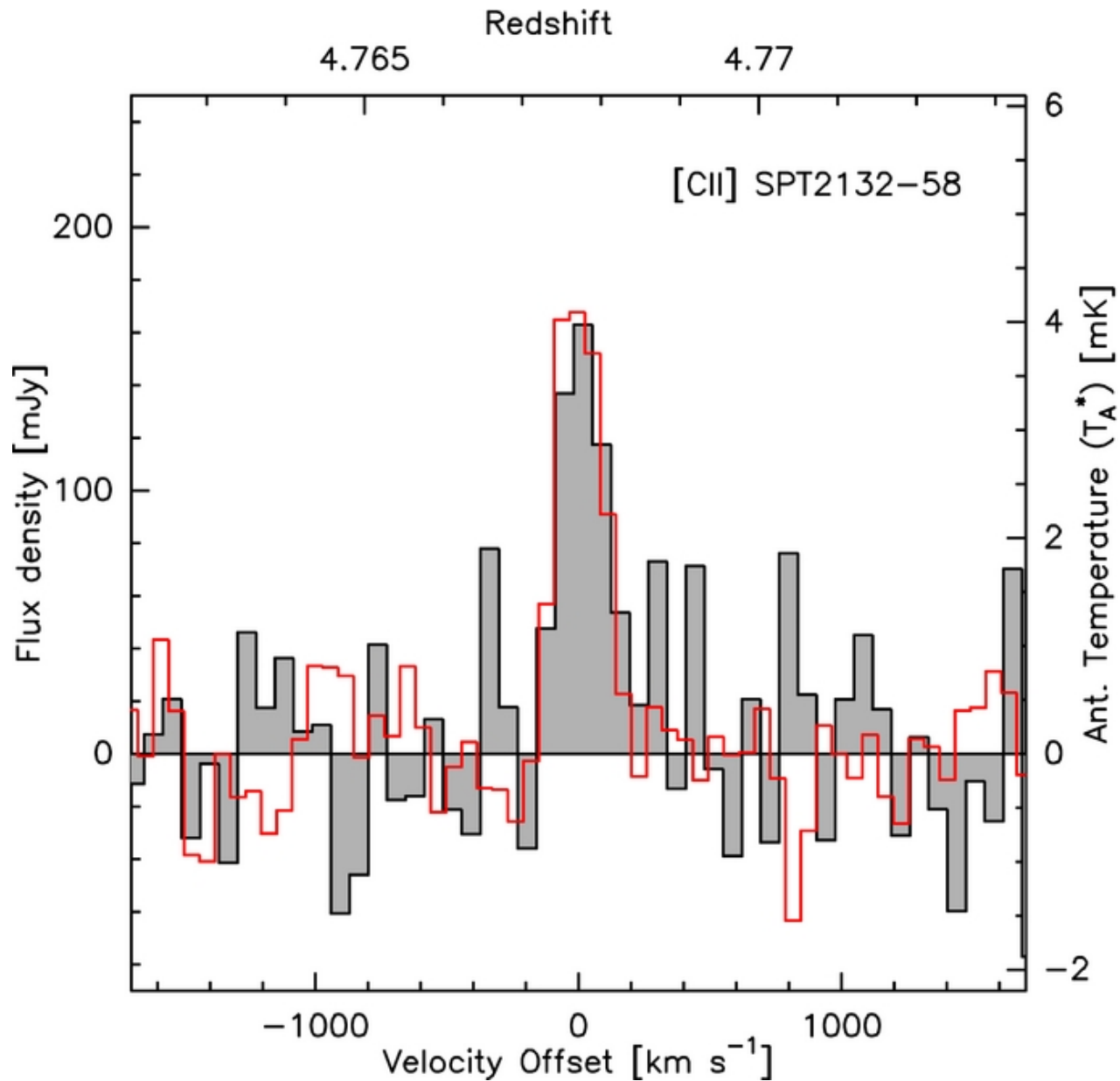
Figure 15. from ALMA Redshifts of Millimeter-selected Galaxies from the SPT Survey: The Redshift Distribution of Dusty Star-forming Galaxies Weiß et al. 2013 ApJ 767 88 doi:10.1088/0004-637X/767/1/88 https://dx.doi.org/10.1088/0004-637X/767/1/88 © 2013. The American Astronomical Society. All rights reserved.
