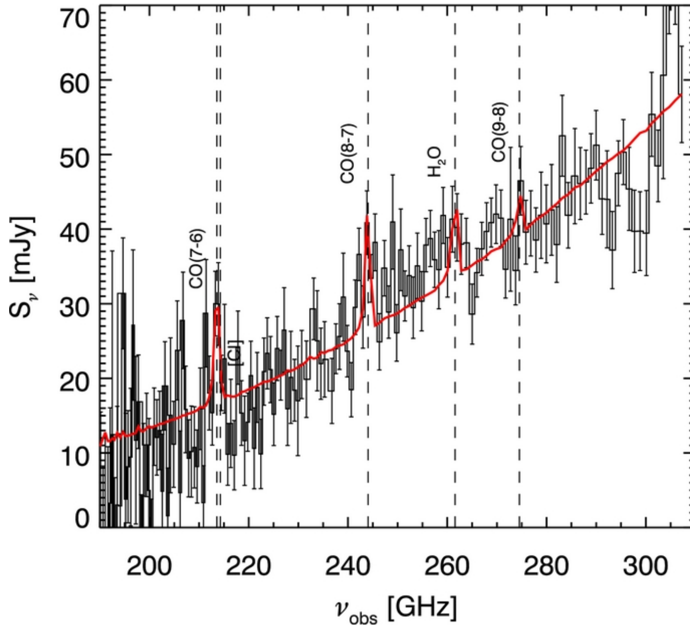
Figure 13. from ALMA Redshifts of Millimeter-selected Galaxies from the SPT Survey: The Redshift Distribution of Dusty Star-forming Galaxies Weiß et al. 2013 ApJ 767 88 doi:10.1088/0004-637X/767/1/88 https://dx.doi.org/10.1088/0004-637X/767/1/88 © 2013. The American Astronomical Society. All rights reserved.
