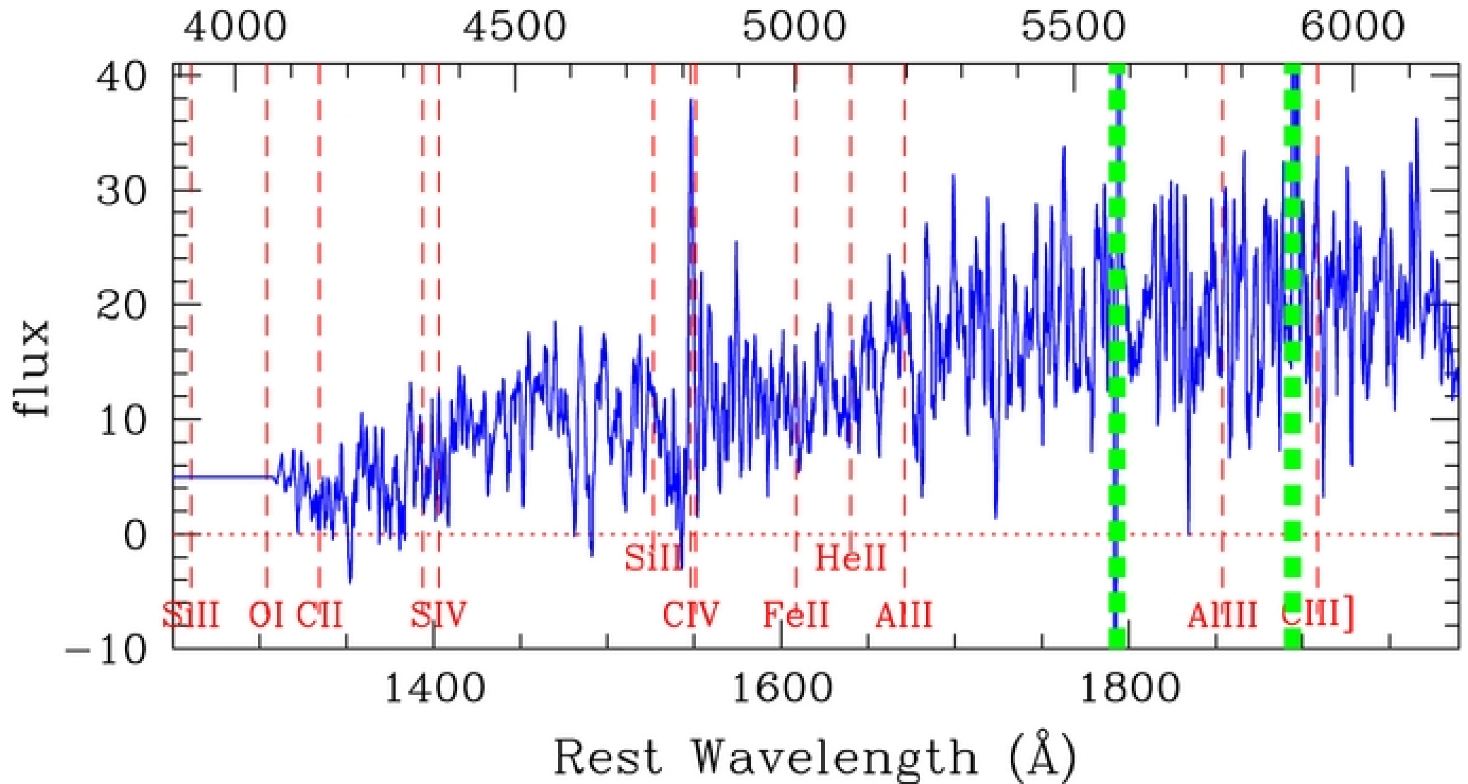
Figure 12. from ALMA Redshifts of Millimeter-selected Galaxies from the SPT Survey: The Redshift Distribution of Dusty Star-forming Galaxies Weiß et al. 2013 ApJ 767 88 doi:10.1088/0004-637X/767/1/88 https://dx.doi.org/10.1088/0004-637X/767/1/88 © 2013. The American Astronomical Society. All rights reserved.
