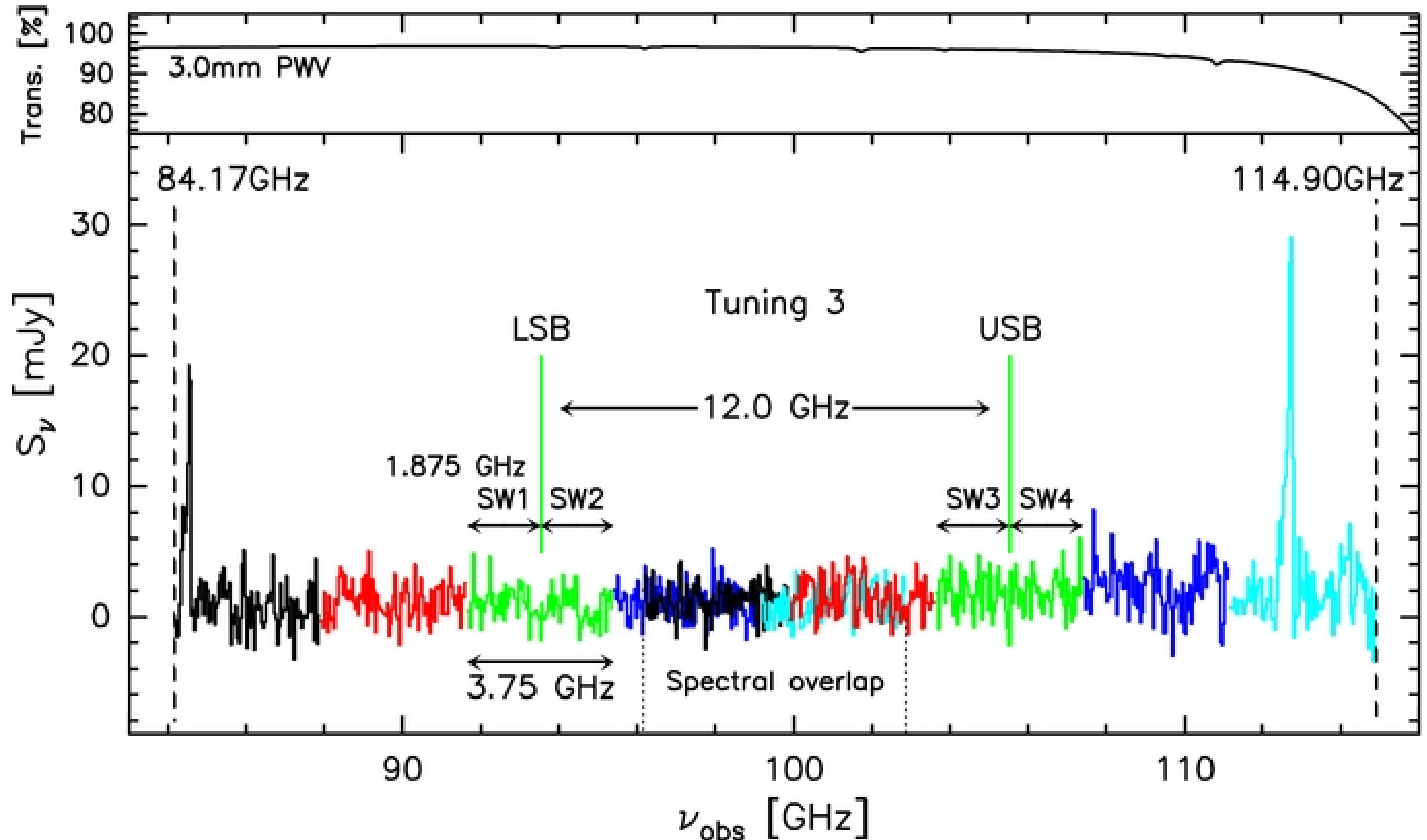
Figure 1. from ALMA Redshifts of Millimeter-selected Galaxies from the SPT Survey: The Redshift Distribution of Dusty Star-forming Galaxies Weiß et al. 2013 ApJ 767 88 doi:10.1088/0004-637X/767/1/88 https://dx.doi.org/10.1088/0004-637X/767/1/88 © 2013. The American Astronomical Society. All rights reserved.
