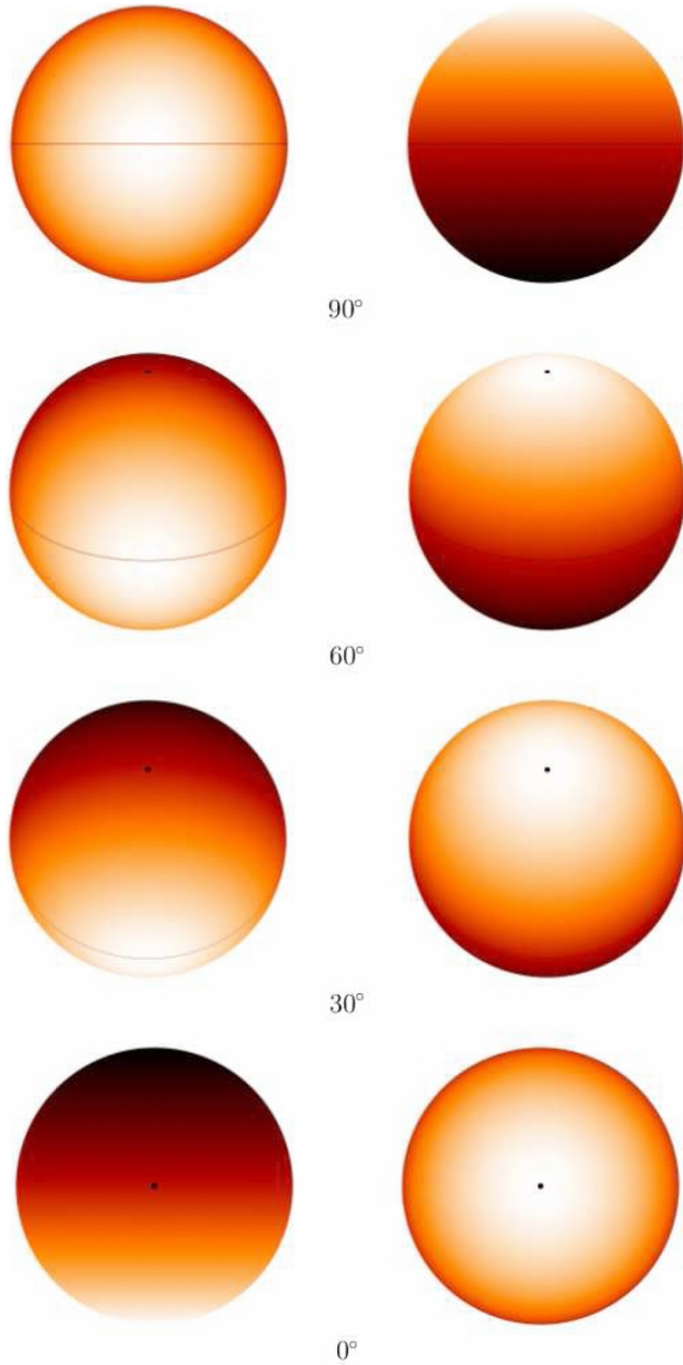
Figure 6. from Asteroseismic Determination of Obliquities of the Exoplanet Systems Kepler-50 and Kepler-65 Chaplin et al. 2013 ApJ 766 101 doi:10.1088/0004-637X/766/2/101 https://dx.doi.org/10.1088/0004-637X/766/2/101 © 2013. The American Astronomical Society. All rights reserved.
