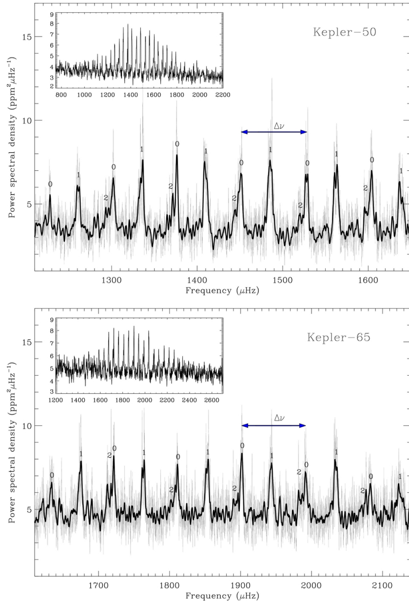
Figure 1. from Asteroseismic Determination of Obliquities of the Exoplanet Systems Kepler-50 and Kepler-65 Chaplin et al. 2013 ApJ 766 101 doi:10.1088/0004-637X/766/2/101 https://dx.doi.org/10.1088/0004-637X/766/2/101 © 2013. The American Astronomical Society. All rights reserved.
