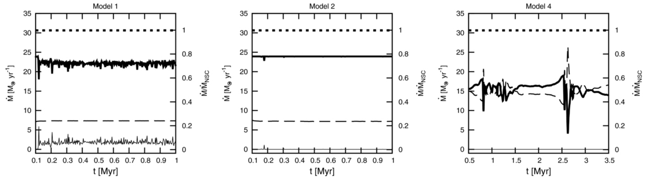
Figure 7. from On the Fate of the Matter Reinserted within Young Nuclear Stellar Clusters Hueyotl-Zahuantitla et al. 2013 ApJ 766 92 doi:10.1088/0004-637X/766/2/92 https://dx.doi.org/10.1088/0004-637X/766/2/92 © 2013. The American Astronomical Society. All rights reserved.
