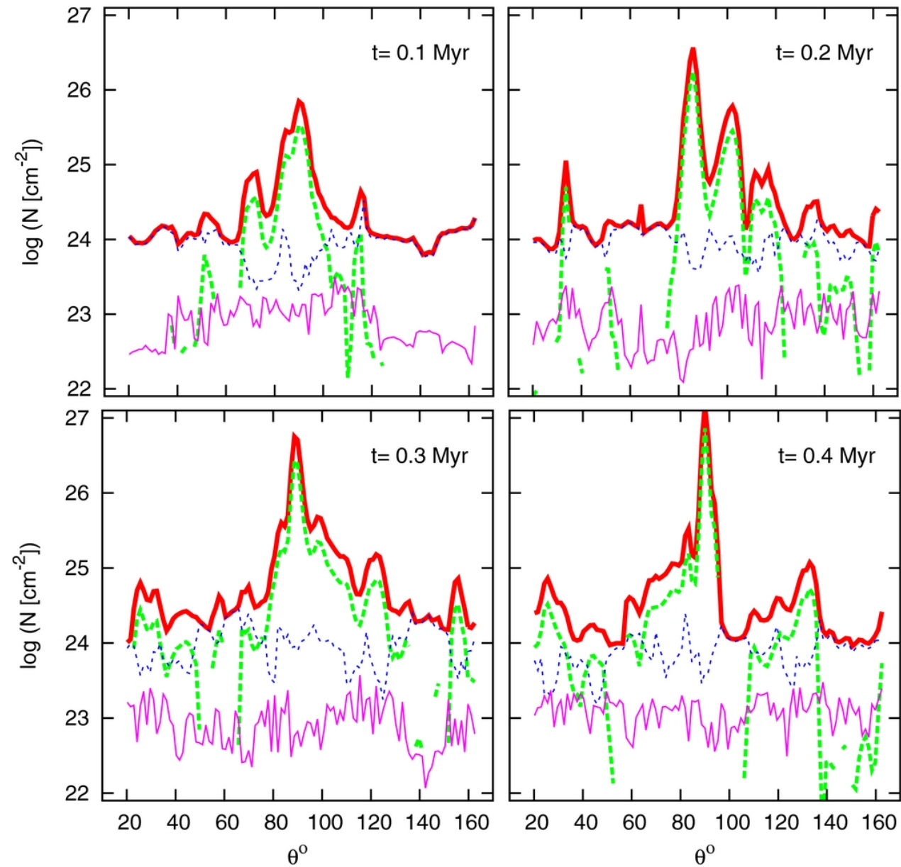
Figure 4. from On the Fate of the Matter Reinserted within Young Nuclear Stellar Clusters Hueyotl-Zahuantitla et al. 2013 ApJ 766 92 doi:10.1088/0004-637X/766/2/92 https://dx.doi.org/10.1088/0004-637X/766/2/92
