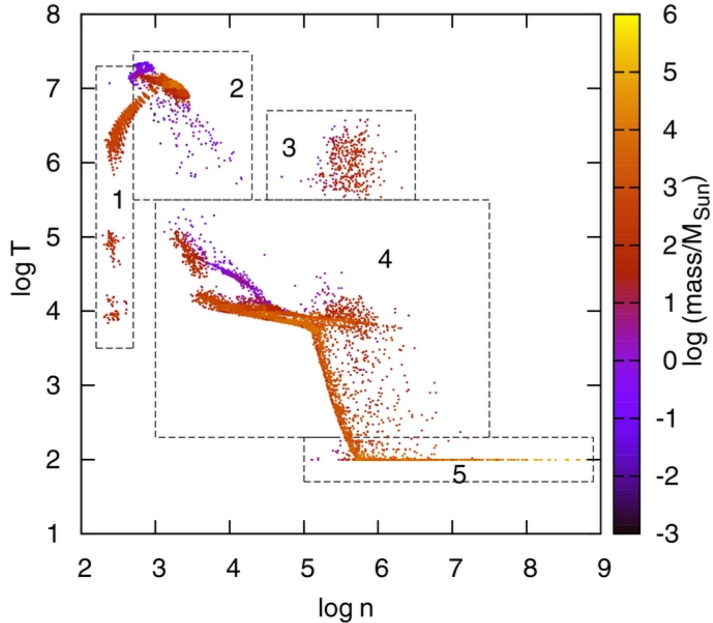
Figure 3. from On the Fate of the Matter Reinserted within Young Nuclear Stellar Clusters Hueyotl-Zahuantitla et al. 2013 ApJ 766 92 doi:10.1088/0004-637X/766/2/92 https://dx.doi.org/10.1088/0004-637X/766/2/92 © 2013. The American Astronomical Society. All rights reserved.
