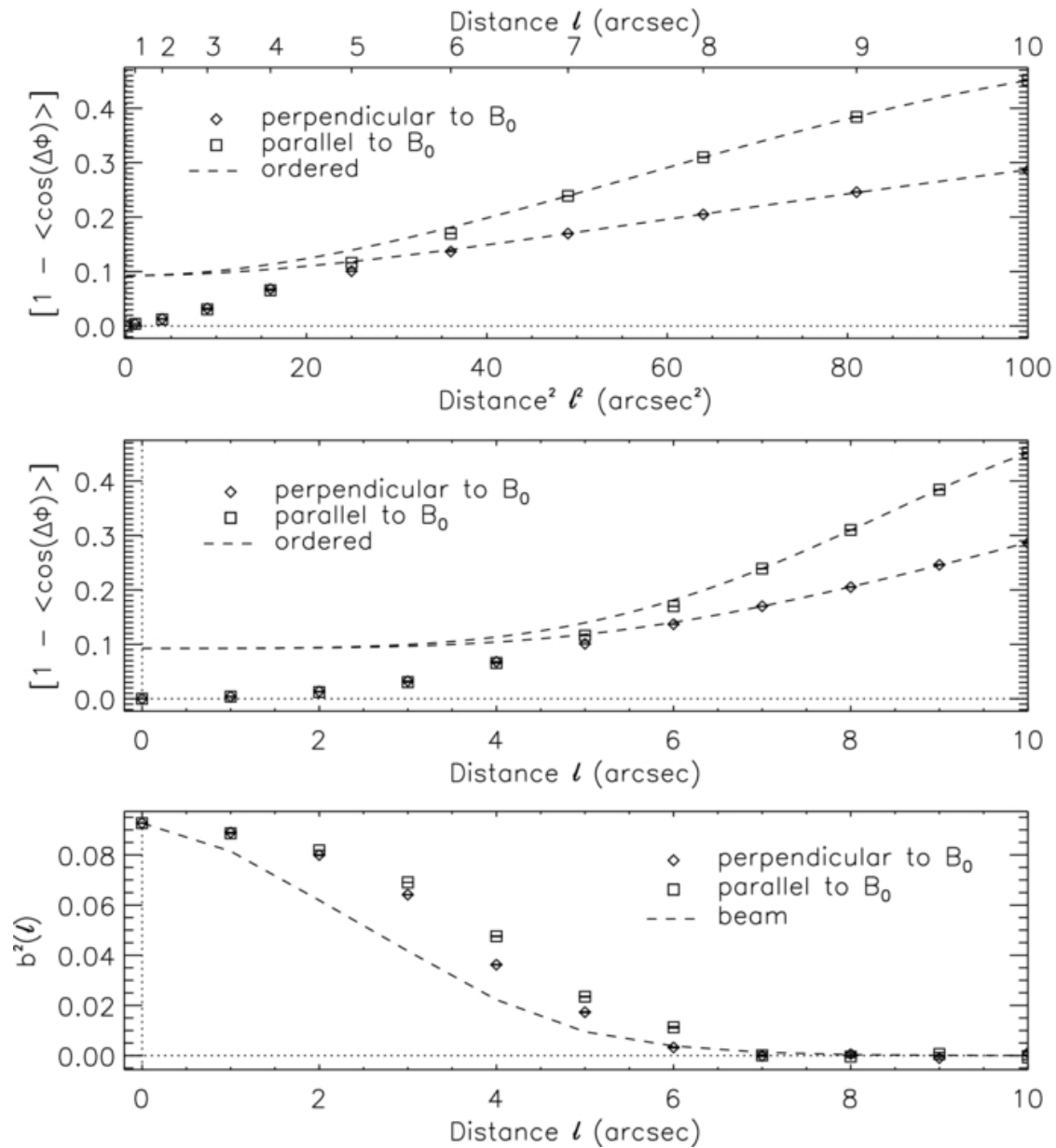
Figure 9. from Characterizing Magnetized Turbulence in M51 Houde et al. 2013 ApJ 766 49 doi:10.1088/0004-637X/766/1/49 https://dx.doi.org/10.1088/0004-637X/766/1/49 © 2013. The American Astronomical Society. All rights reserved.
