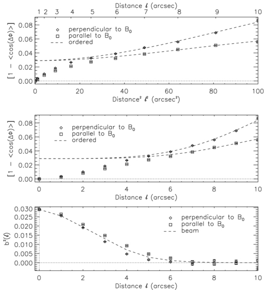
Figure 8. from Characterizing Magnetized Turbulence in M51 Houde et al. 2013 ApJ 766 49 doi:10.1088/0004-637X/766/1/49 https://dx.doi.org/10.1088/0004-637X/766/1/49 © 2013. The American Astronomical Society. All rights reserved.
