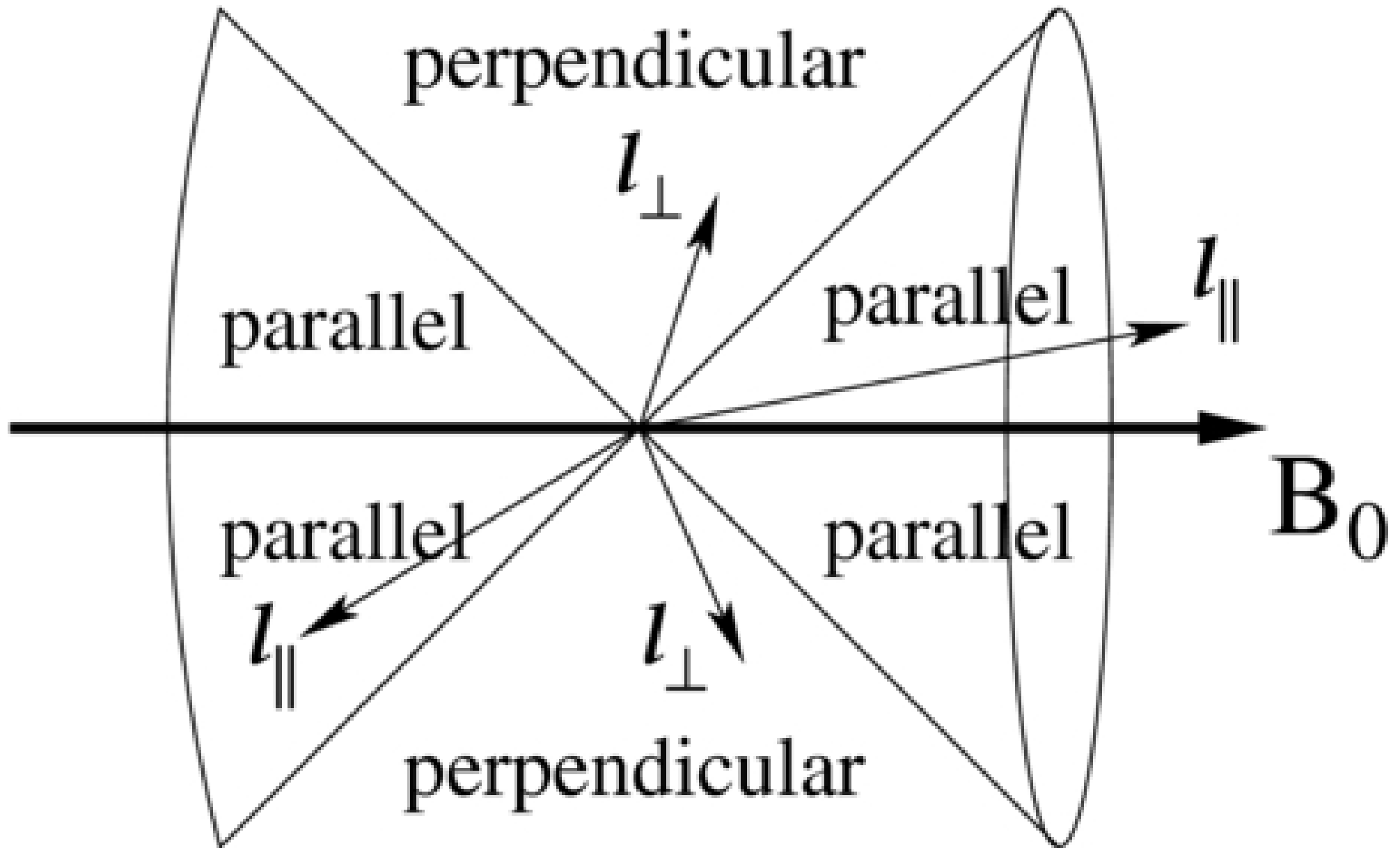
Figure 7. from Characterizing Magnetized Turbulence in M51 Houde et al. 2013 ApJ 766 49 doi:10.1088/0004-637X/766/1/49 https://dx.doi.org/10.1088/0004-637X/766/1/49 © 2013. The American Astronomical Society. All rights reserved.
