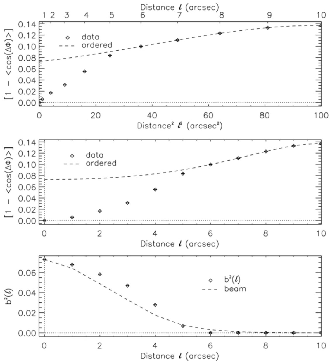
Figure 6. from Characterizing Magnetized Turbulence in M51 Houde et al. 2013 ApJ 766 49 doi:10.1088/0004-637X/766/1/49 https://dx.doi.org/10.1088/0004-637X/766/1/49 © 2013. The American Astronomical Society. All rights reserved.
