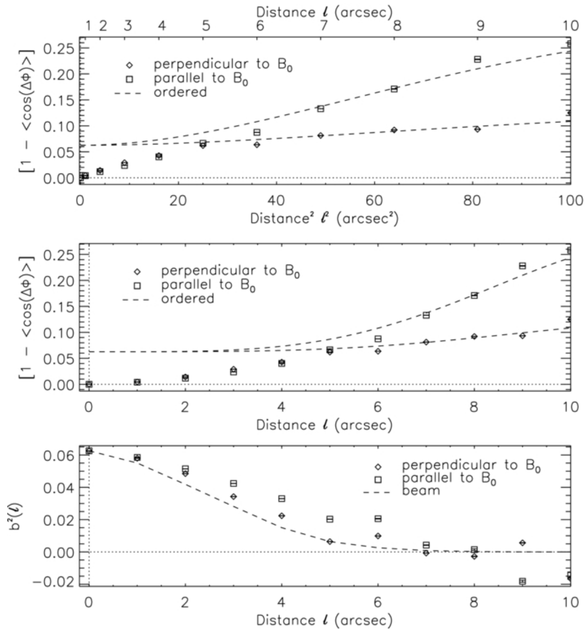
Figure 12. from Characterizing Magnetized Turbulence in M51 Houde et al. 2013 ApJ 766 49 doi:10.1088/0004-637X/766/1/49 https://dx.doi.org/10.1088/0004-637X/766/1/49 © 2013. The American Astronomical Society. All rights reserved.
