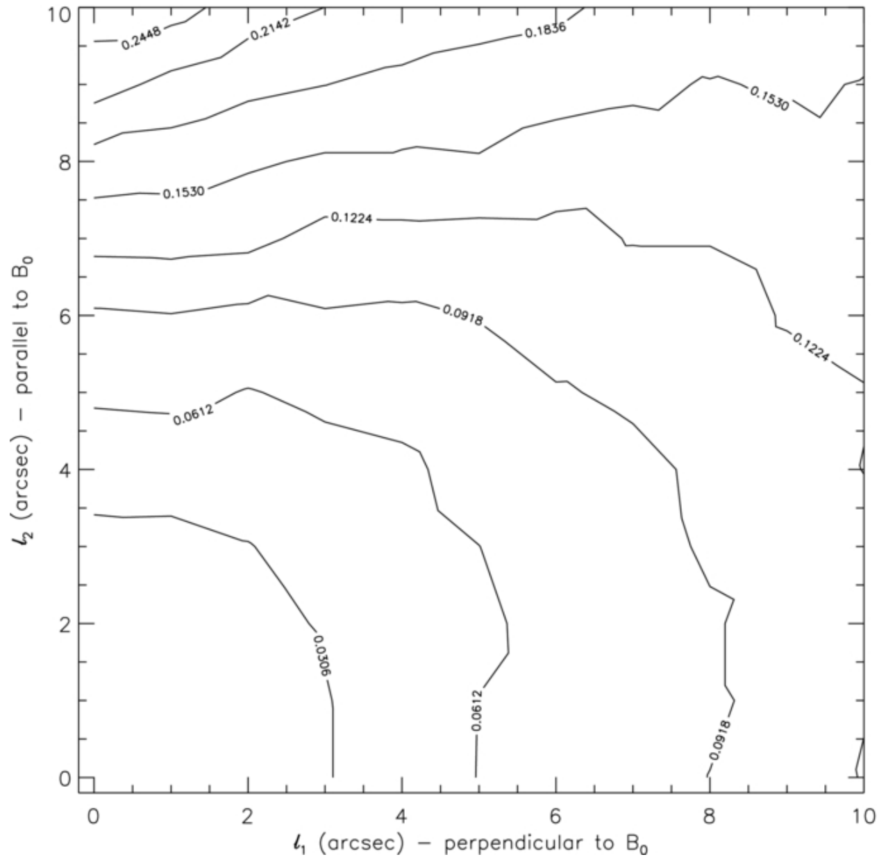
Figure 11. from Characterizing Magnetized Turbulence in M51 Houde et al. 2013 ApJ 766 49 doi:10.1088/0004-637X/766/1/49 https://dx.doi.org/10.1088/0004-637X/766/1/49
