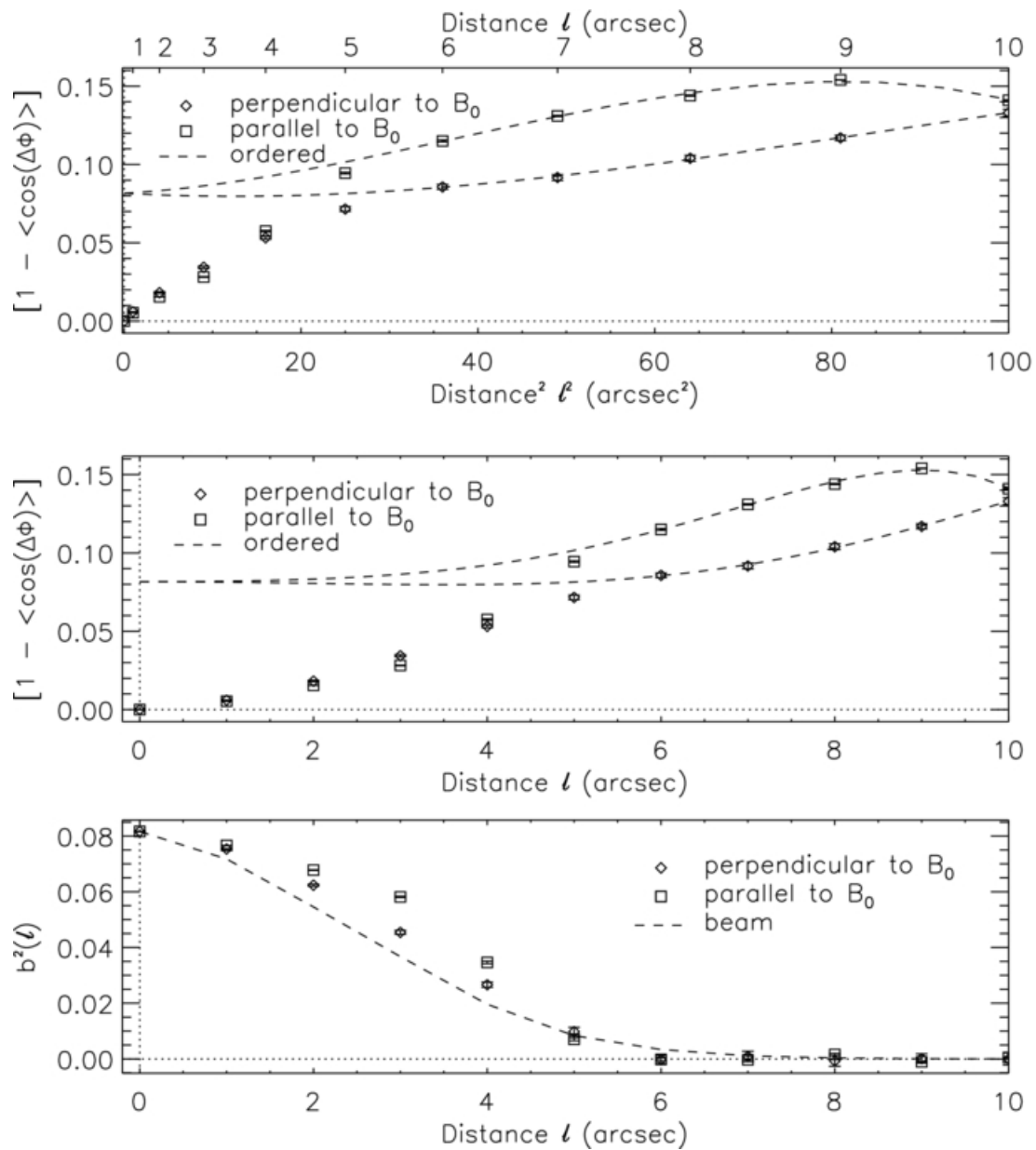
Figure 10. from Characterizing Magnetized Turbulence in M51 Houde et al. 2013 ApJ 766 49 doi:10.1088/0004-637X/766/1/49 https://dx.doi.org/10.1088/0004-637X/766/1/49
